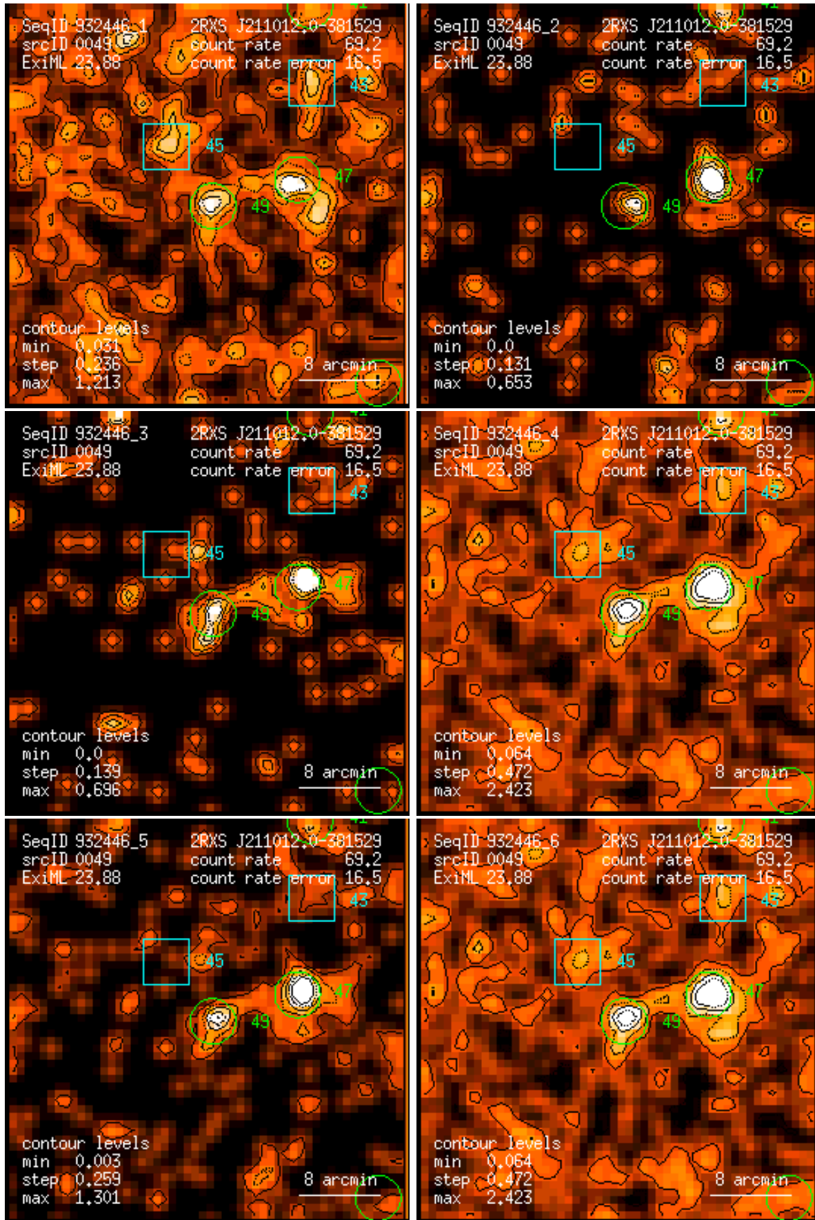
Figure 49: RASS 932446: detection 0049: band rate images, Gaussian filter: (1) PSPC channels 11 – 41, (2) 52 – 90, (3) 91 – 201, (4) 11 – 235, (5) 52 – 201, (6) 11 – 201. Broad band rates in counts/ks. Band rate contour levels in counts/ks/arcmin 2 .
