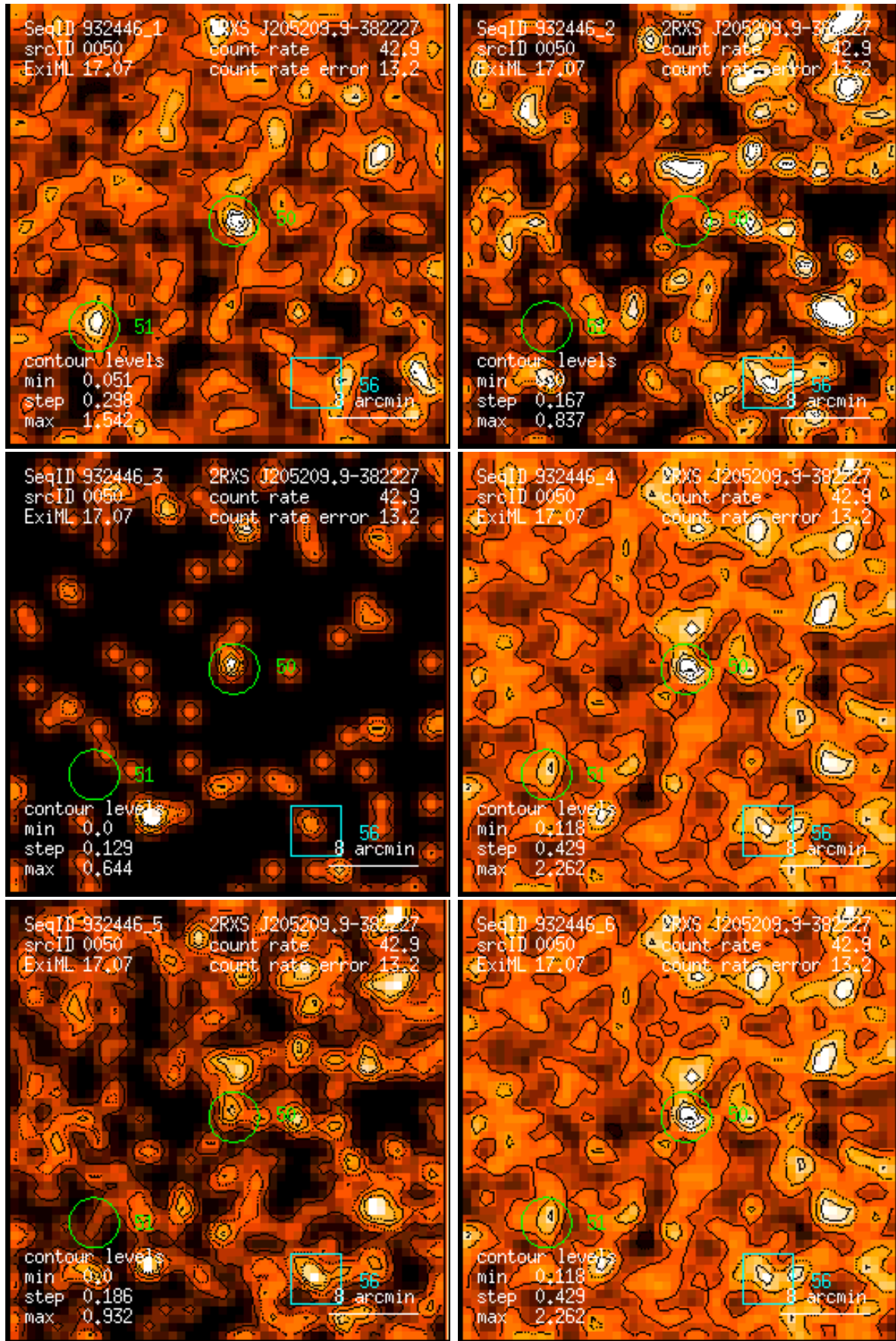
Figure 50: RASS 932446: detection 0050: band rate images, Gaussian filter: (1) PSPC channels 11 – 41, (2) 52 – 90, (3) 91 – 201, (4) 11 – 235, (5) 52 – 201, (6) 11 – 201. Broad band rates in counts/ks. Band rate contour levels in counts/ks/arcmin 2 .
