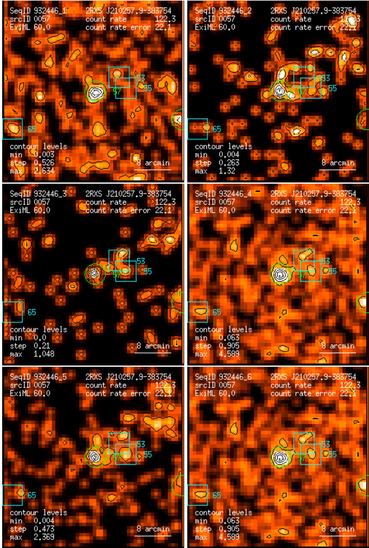
Figure 57: RASS 932446: detection 0057: band rate images, Gaussian filter: (1) PSPC channels 11 – 41, (2) 52 – 90, (3) 91 – 201, (4) 11 – 235, (5) 52 – 201, (6) 11 – 201. Broad band rates in counts/ks. Band rate contour levels in counts/ks/arcmin 2 .
