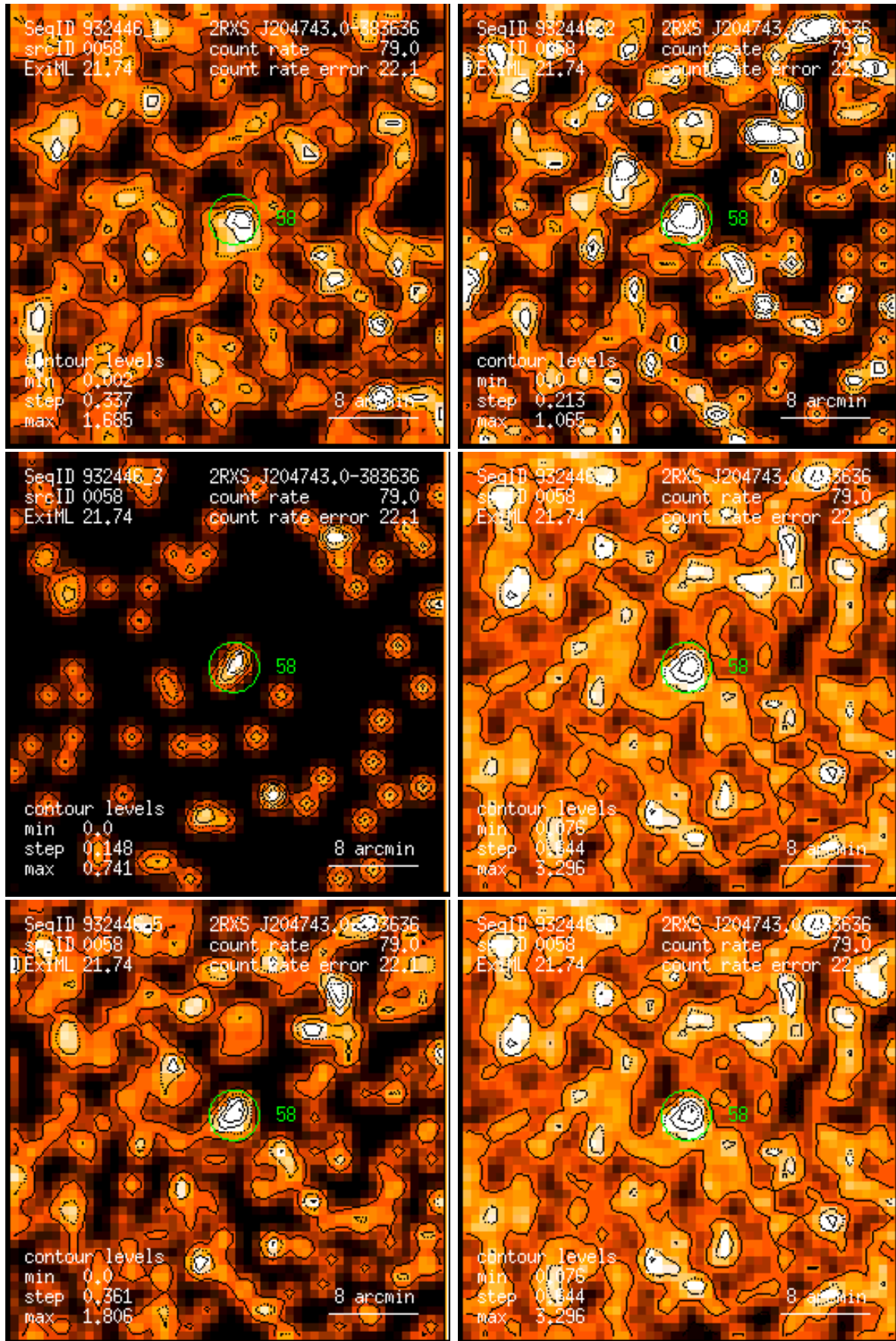
Figure 58: RASS 932446: detection 0058: band rate images, Gaussian filter: (1) PSPC channels 11 – 41, (2) 52 – 90, (3) 91 – 201, (4) 11 – 235, (5) 52 – 201, (6) 11 – 201. Broad band rates in counts/ks. Band rate contour levels in counts/ks/arcmin 2 .
