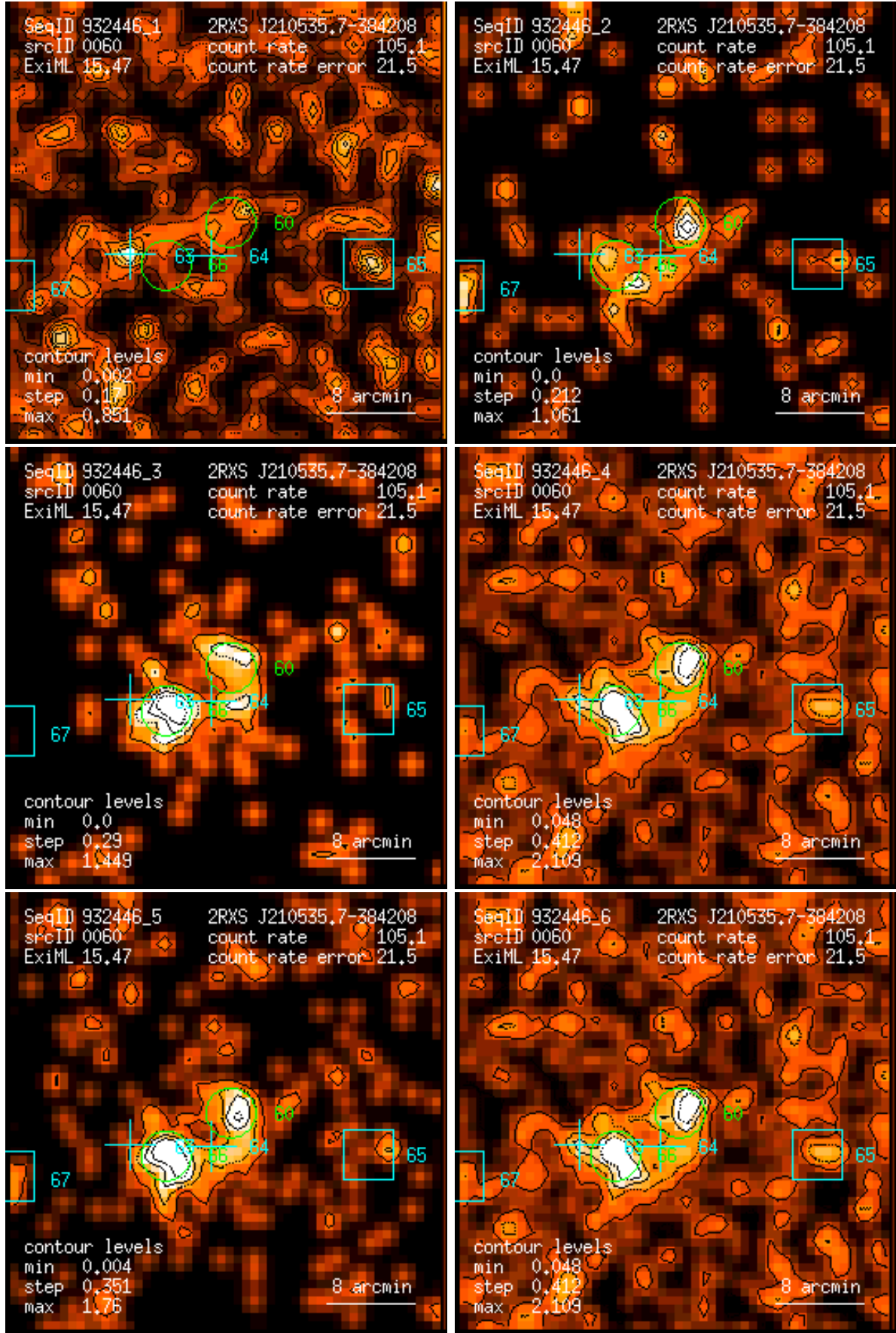
Figure 60: RASS 932446: detection 0060: band rate images, Gaussian filter: (1) PSPC channels 11 – 41, (2) 52 – 90, (3) 91 – 201, (4) 11 – 235, (5) 52 – 201, (6) 11 – 201. Broad band rates in counts/ks. Band rate contour levels in counts/ks/arcmin 2 .
