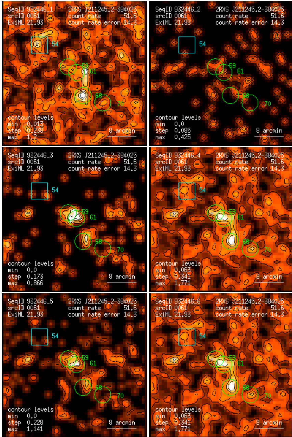
Figure 61: RASS 932446: detection 0061: band rate images, Gaussian filter: (1) PSPC channels 11 – 41, (2) 52 – 90, (3) 91 – 201, (4) 11 – 235, (5) 52 – 201, (6) 11 – 201. Broad band rates in counts/ks. Band rate contour levels in counts/ks/arcmin 2 .
