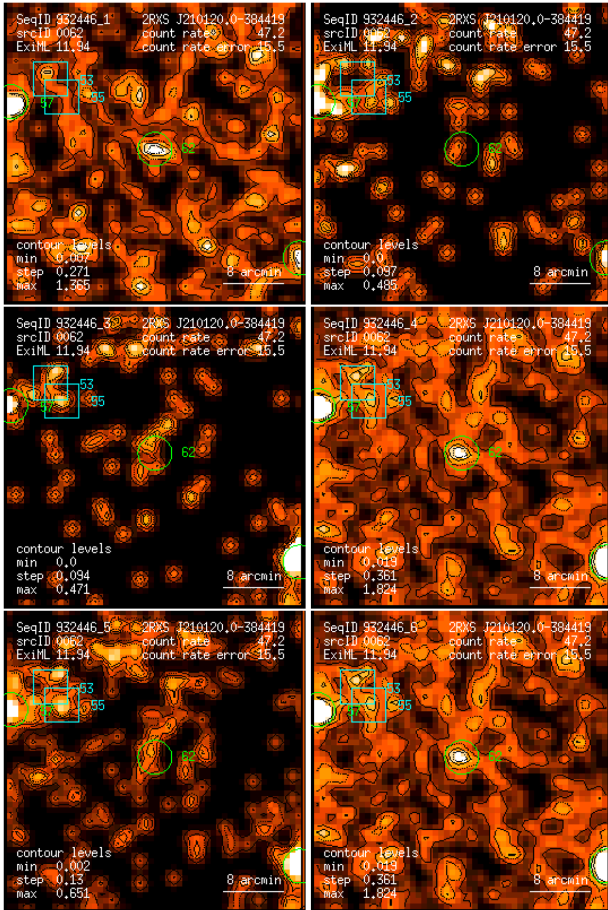
Figure 62: RASS 932446: detection 0062: band rate images, Gaussian filter: (1) PSPC channels 11 – 41, (2) 52 – 90, (3) 91 – 201, (4) 11 – 235, (5) 52 – 201, (6) 11 – 201. Broad band rates in counts/ks. Band rate contour levels in counts/ks/arcmin 2 .
