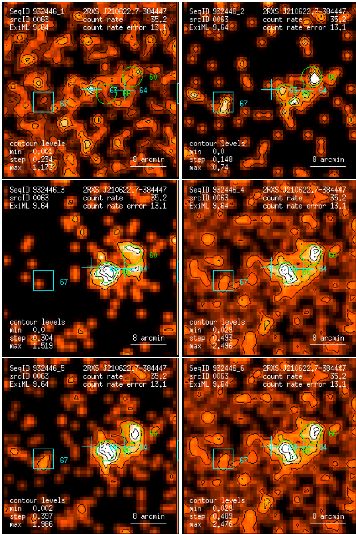
Figure 63: RASS 932446: detection 0063: band rate images, Gaussian filter: (1) PSPC channels 11 – 41, (2) 52 – 90, (3) 91 – 201, (4) 11 – 235, (5) 52 – 201, (6) 11 – 201. Broad band rates in counts/ks. Band rate contour levels in counts/ks/arcmin 2 .
