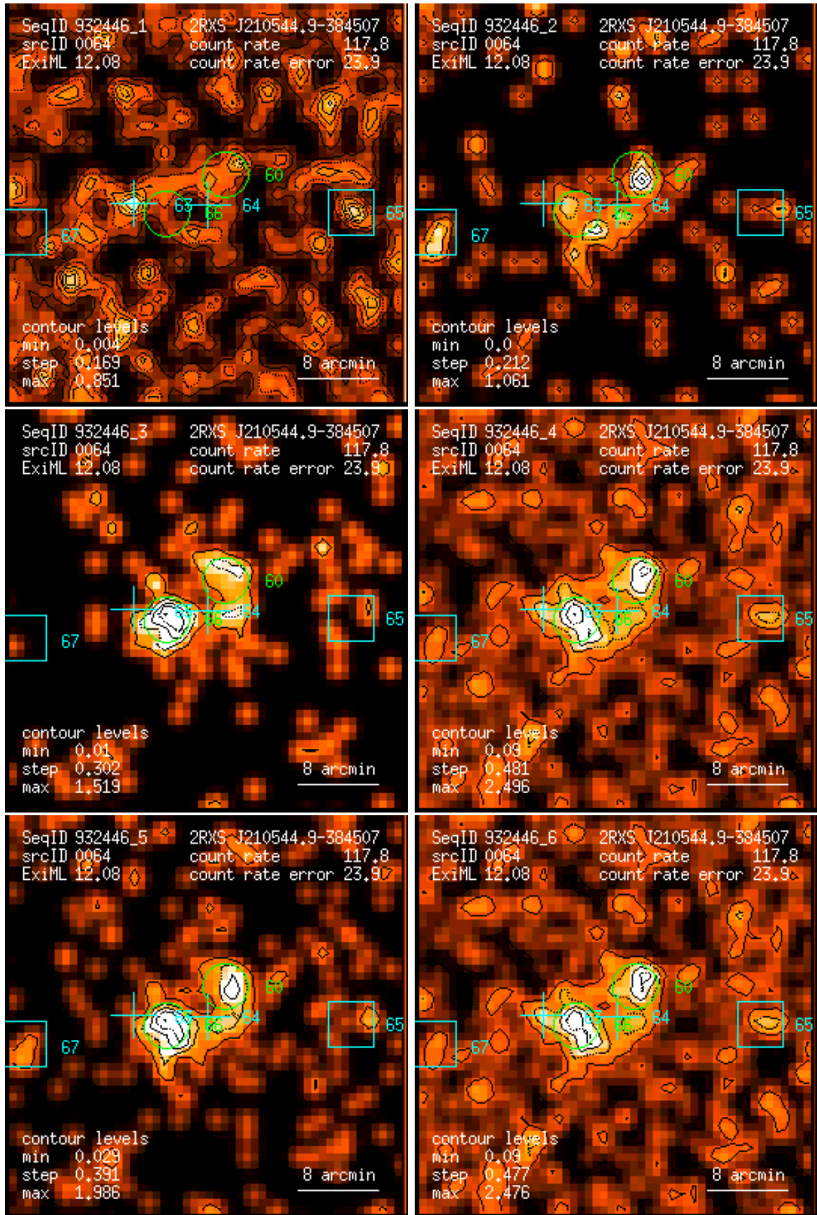
Figure 64: RASS 932446: detection 0064: band rate images, Gaussian filter: (1) PSPC channels 11 – 41, (2) 52 – 90, (3) 91 – 201, (4) 11 – 235, (5) 52 – 201, (6) 11 – 201. Broad band rates in counts/ks. Band rate contour levels in counts/ks/arcmin 2 .
