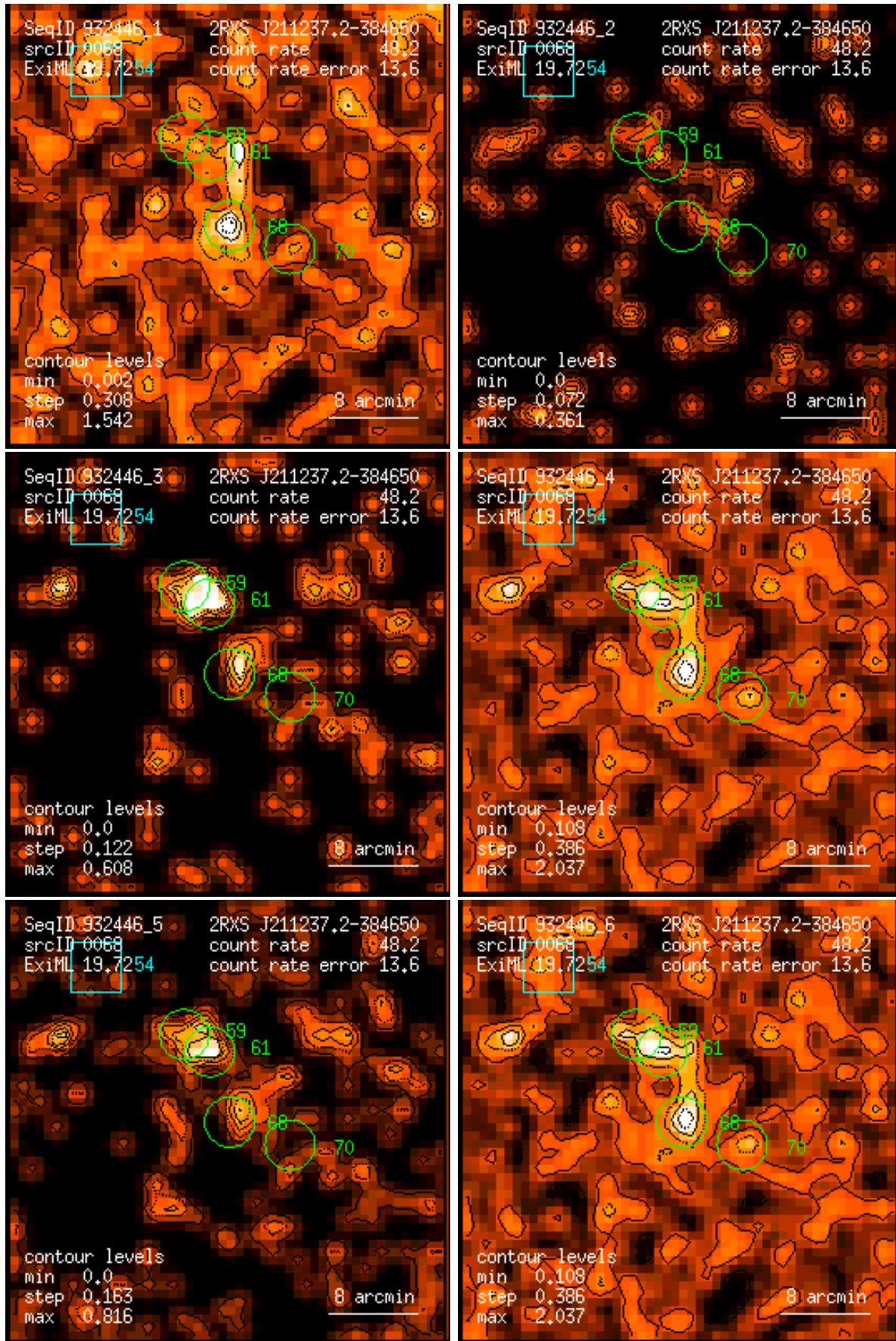
Figure 68: RASS 932446: detection 0068: band rate images, Gaussian filter: (1) PSPC channels 11 – 41, (2) 52 – 90, (3) 91 – 201, (4) 11 – 235, (5) 52 – 201, (6) 11 – 201. Broad band rates in counts/ks. Band rate contour levels in counts/ks/arcmin 2 .
