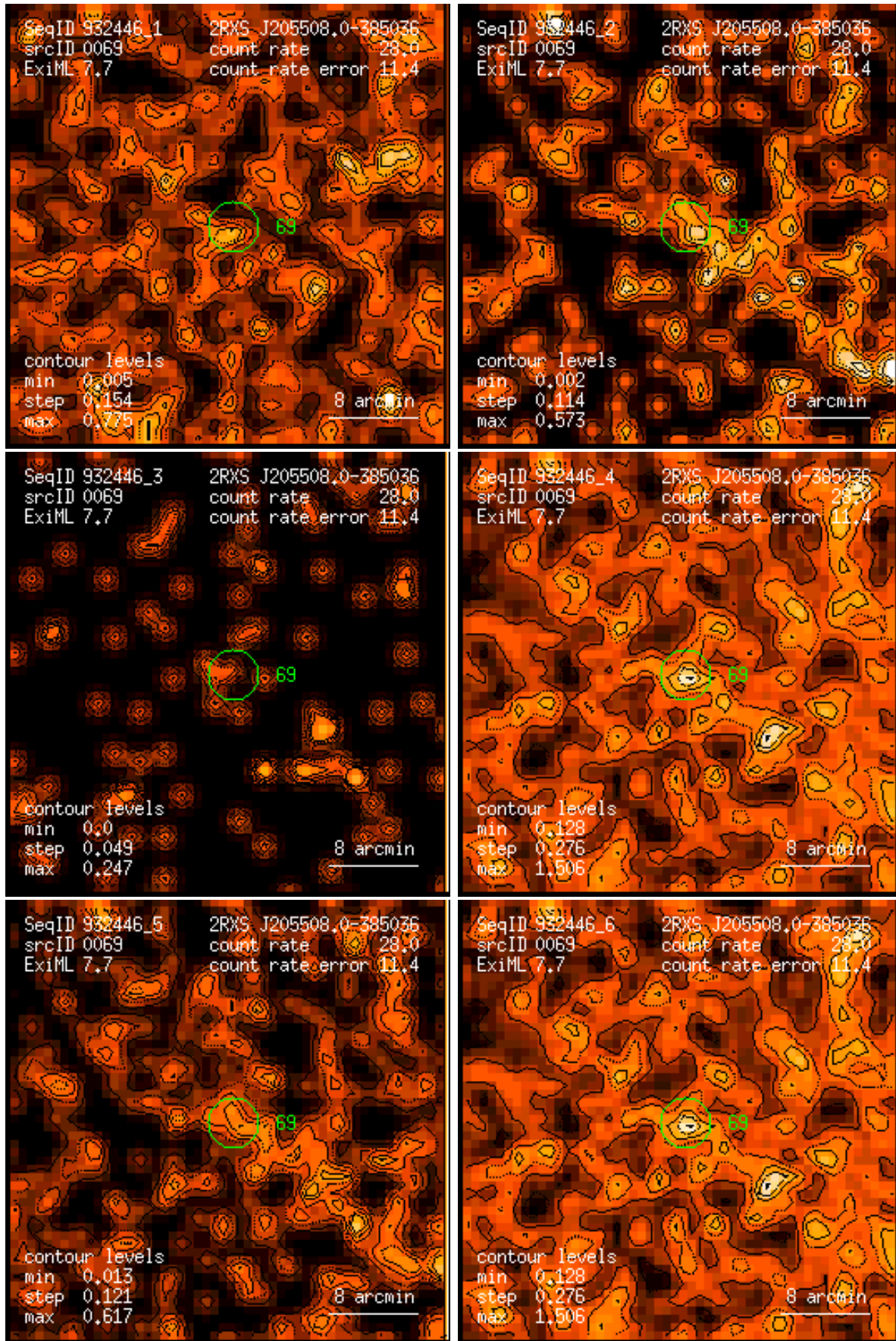
Figure 69: RASS 932446: detection 0069: band rate images, Gaussian filter: (1) PSPC channels 11 – 41, (2) 52 – 90, (3) 91 – 201, (4) 11 – 235, (5) 52 – 201, (6) 11 – 201. Broad band rates in counts/ks. Band rate contour levels in counts/ks/arcmin 2 .
