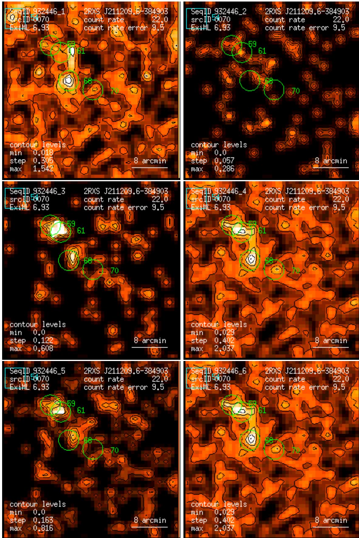
Figure 70: RASS 932446: detection 0070: band rate images, Gaussian filter: (1) PSPC channels 11 – 41, (2) 52 – 90, (3) 91 – 201, (4) 11 – 235, (5) 52 – 201, (6) 11 – 201. Broad band rates in counts/ks. Band rate contour levels in counts/ks/arcmin 2 .
