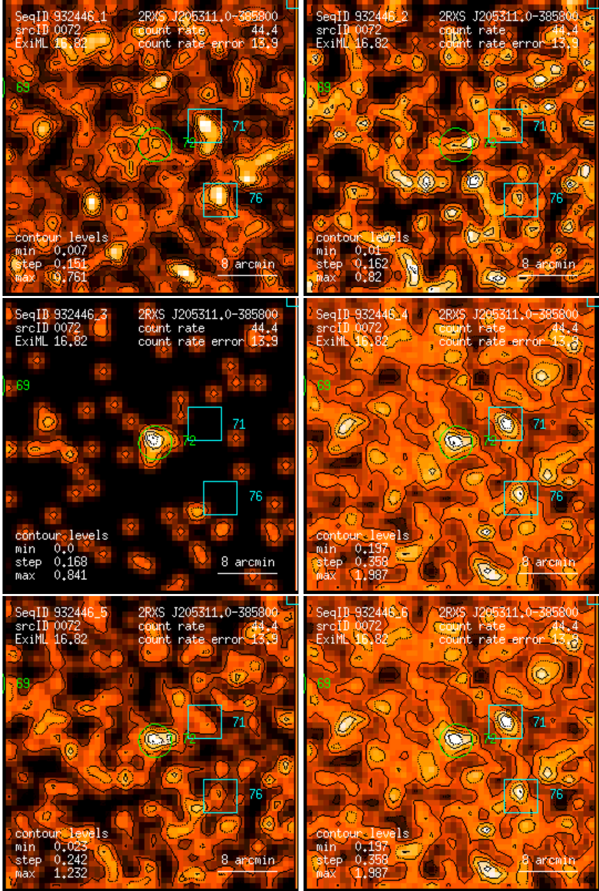
Figure 72: RASS 932446: detection 0072: band rate images, Gaussian filter: (1) PSPC channels 11 – 41, (2) 52 – 90, (3) 91 – 201, (4) 11 – 235, (5) 52 – 201, (6) 11 – 201. Broad band rates in counts/ks. Band rate contour levels in counts/ks/arcmin 2 .
