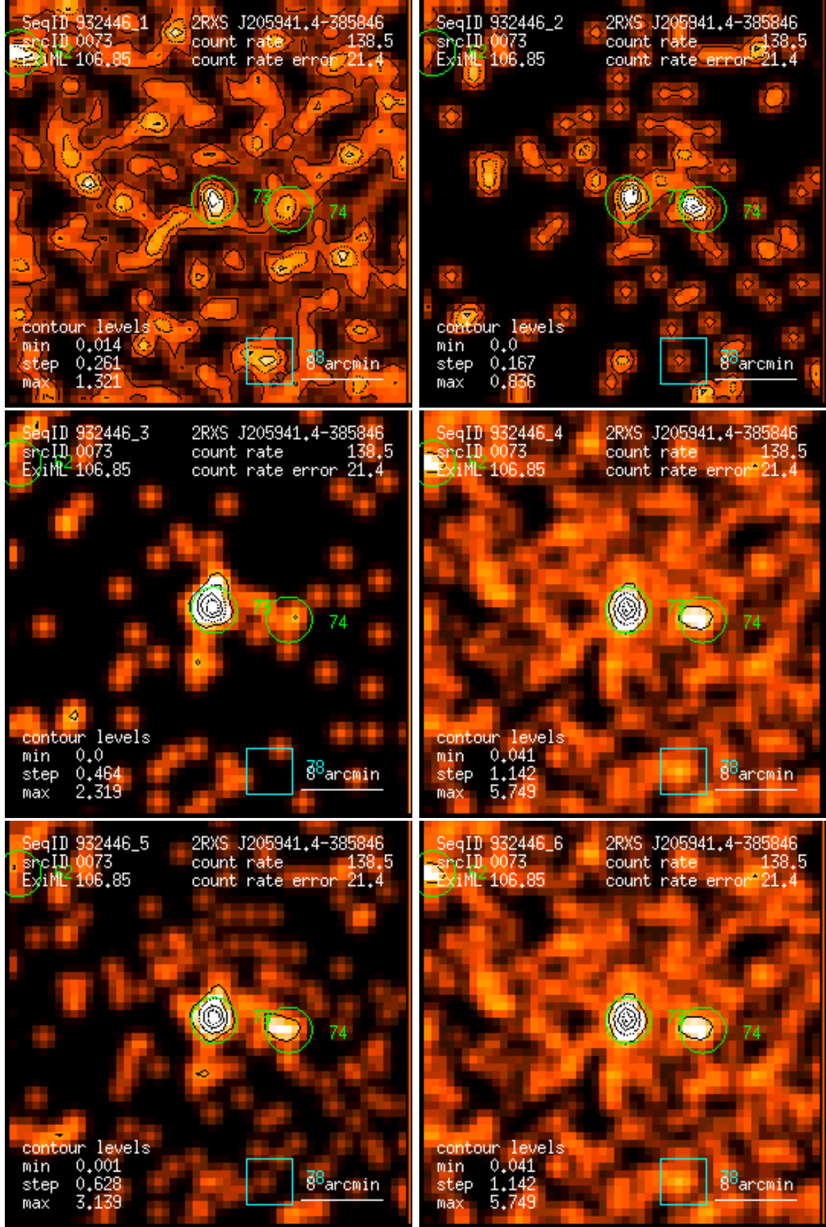
Figure 73: RASS 932446: detection 0073: band rate images, Gaussian filter: (1) PSPC channels 11 – 41, (2) 52 – 90, (3) 91 – 201, (4) 11 – 235, (5) 52 – 201, (6) 11 – 201. Broad band rates in counts/ks. Band rate contour levels in counts/ks/arcmin 2 .
