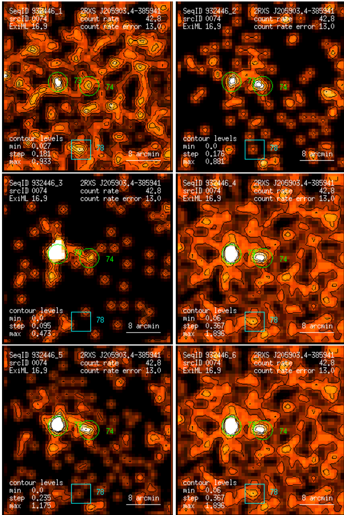
Figure 74: RASS 932446: detection 0074: band rate images, Gaussian filter: (1) PSPC channels 11 – 41, (2) 52 – 90, (3) 91 – 201, (4) 11 – 235, (5) 52 – 201, (6) 11 – 201. Broad band rates in counts/ks. Band rate contour levels in counts/ks/arcmin 2 .
