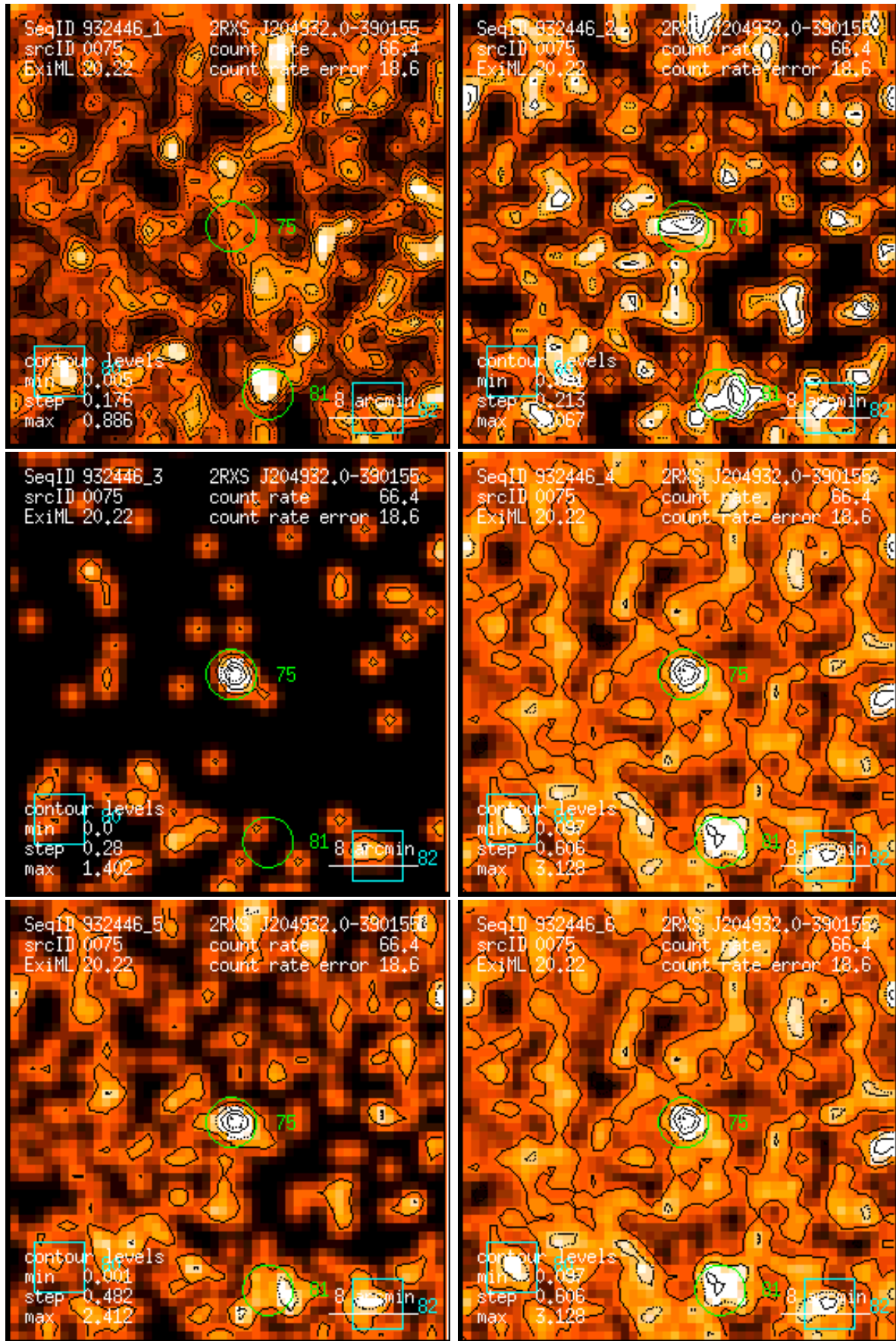
Figure 75: RASS 932446: detection 0075: band rate images, Gaussian filter: (1) PSPC channels 11 – 41, (2) 52 – 90, (3) 91 – 201, (4) 11 – 235, (5) 52 – 201, (6) 11 – 201. Broad band rates in counts/ks. Band rate contour levels in counts/ks/arcmin 2 .
