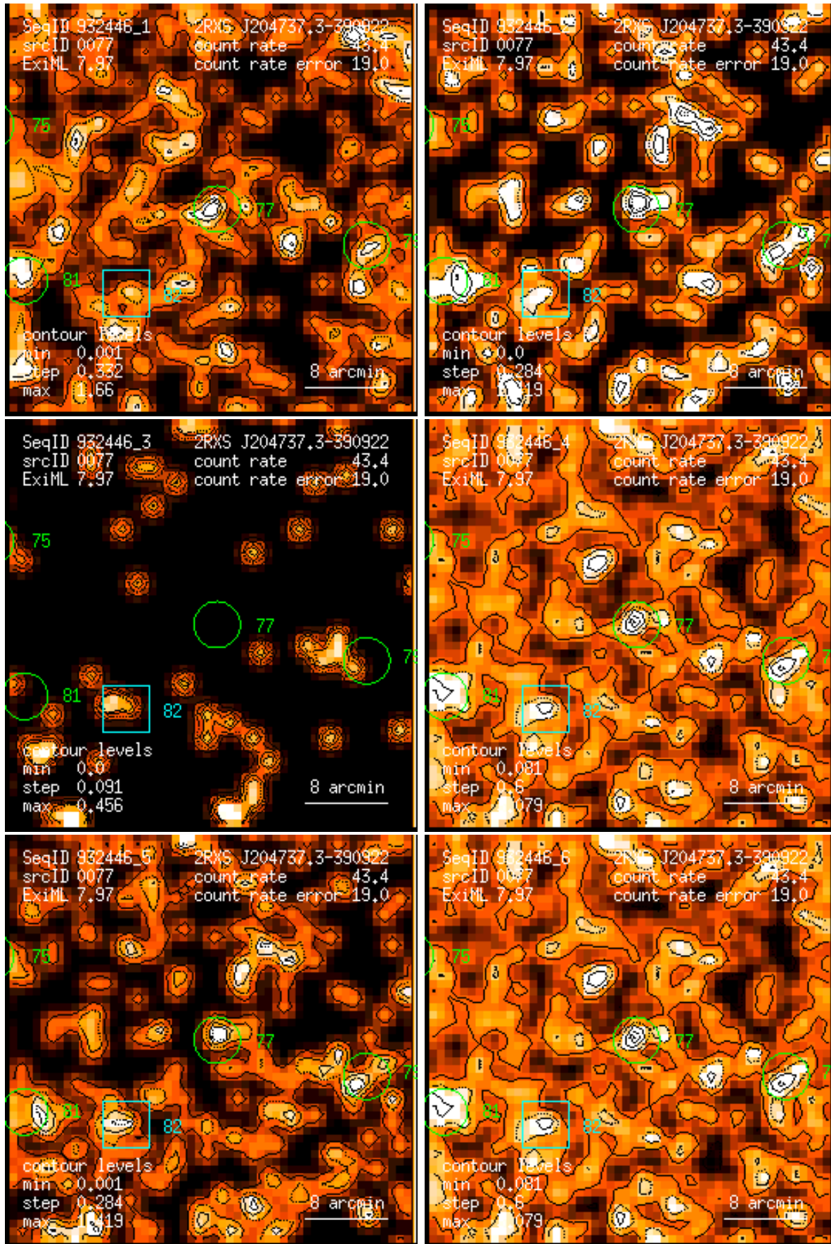
Figure 77: RASS 932446: detection 0077: band rate images, Gaussian filter: (1) PSPC channels 11 – 41, (2) 52 – 90, (3) 91 – 201, (4) 11 – 235, (5) 52 – 201, (6) 11 – 201. Broad band rates in counts/ks. Band rate contour levels in counts/ks/arcmin 2 .
