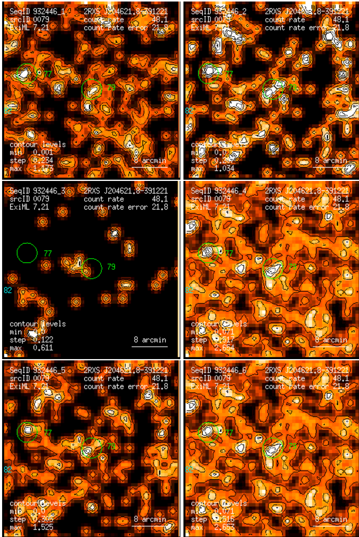
Figure 79: RASS 932446: detection 0079: band rate images, Gaussian filter: (1) PSPC channels 11 – 41, (2) 52 – 90, (3) 91 – 201, (4) 11 – 235, (5) 52 – 201, (6) 11 – 201. Broad band rates in counts/ks. Band rate contour levels in counts/ks/arcmin 2 .
