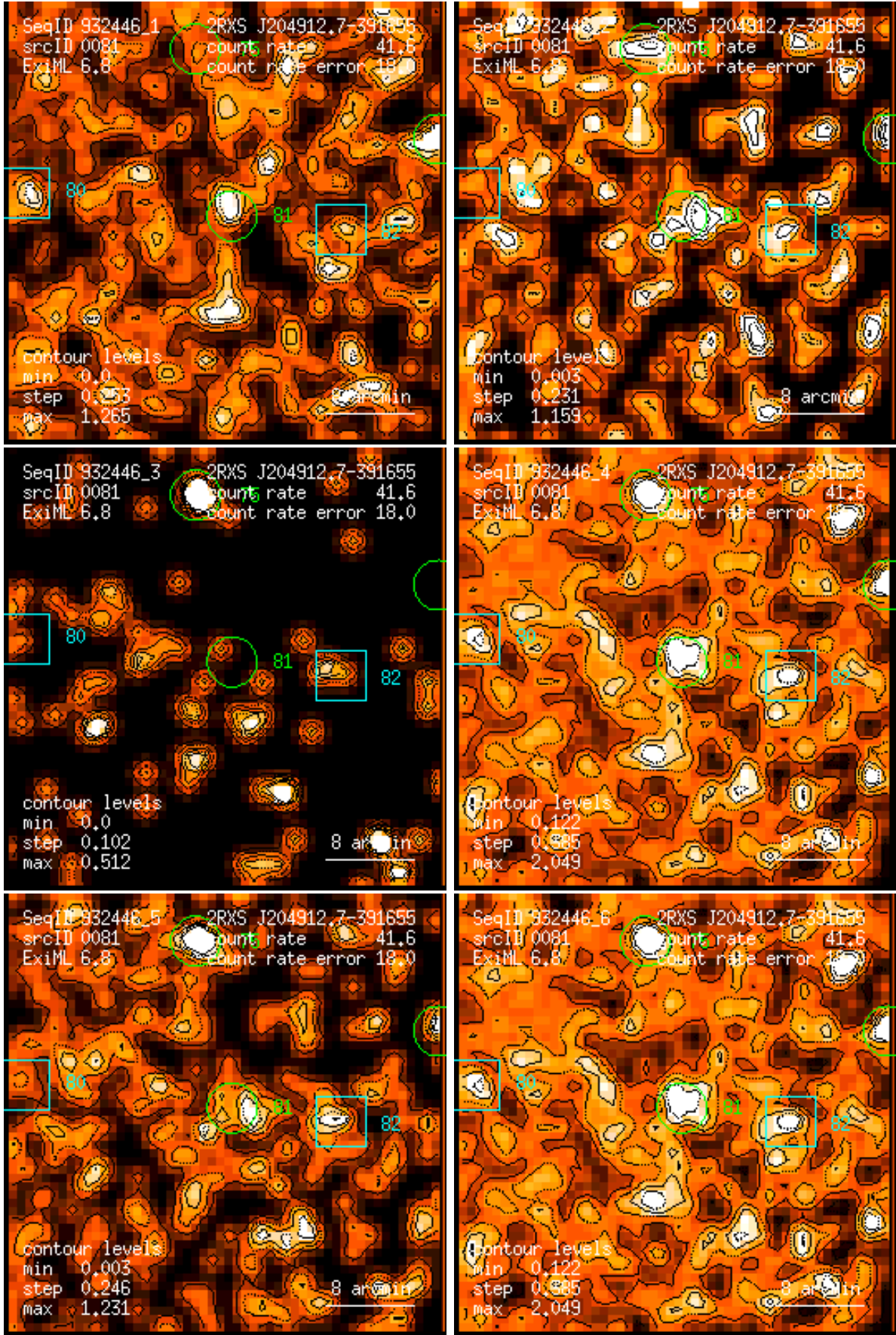
Figure 81: RASS 932446: detection 0081: band rate images, Gaussian filter: (1) PSPC channels 11 – 41, (2) 52 – 90, (3) 91 – 201, (4) 11 – 235, (5) 52 – 201, (6) 11 – 201. Broad band rates in counts/ks. Band rate contour levels in counts/ks/arcmin 2 .
