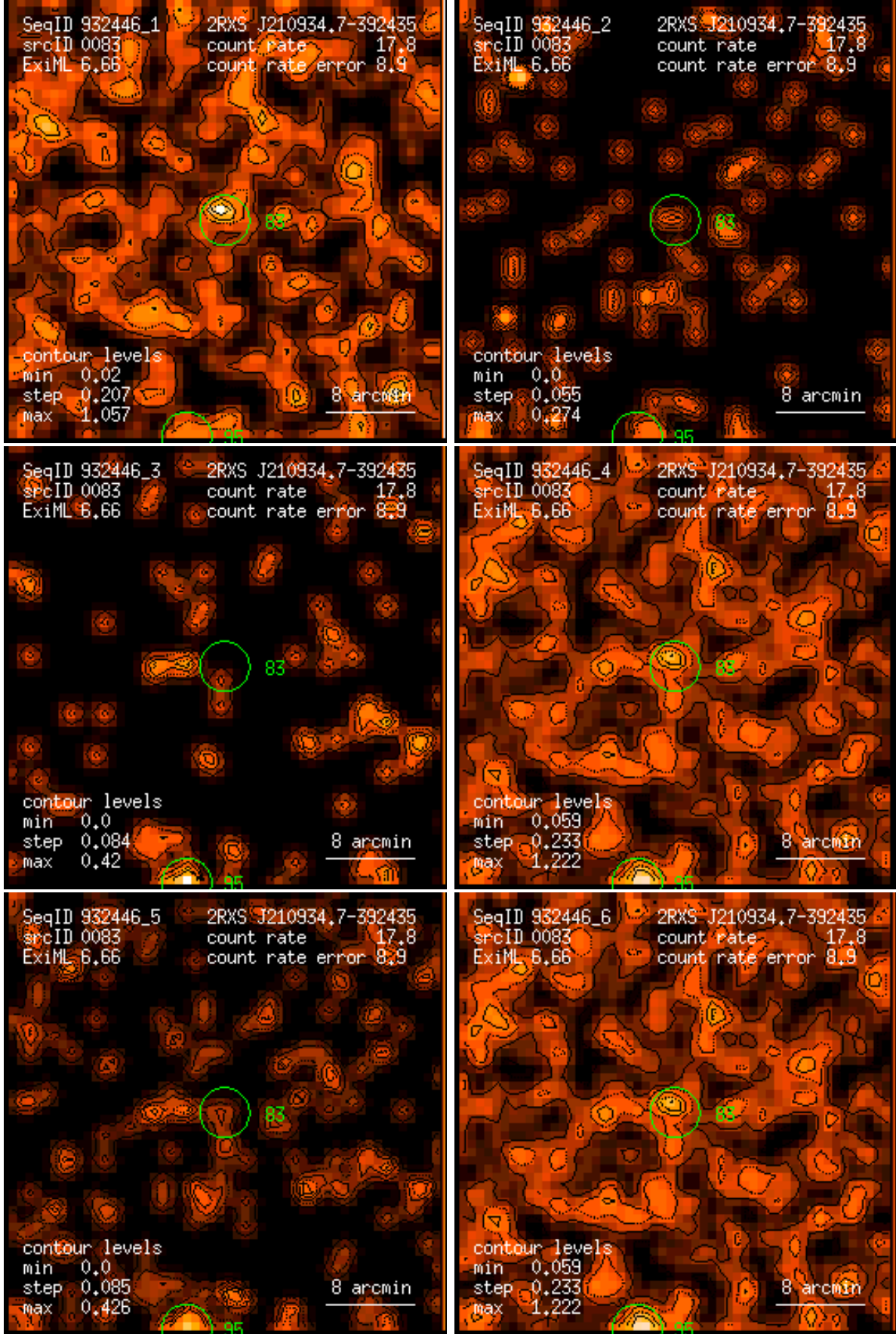
Figure 83: RASS 932446: detection 0083: band rate images, Gaussian filter: (1) PSPC channels 11 – 41, (2) 52 – 90, (3) 91 – 201, (4) 11 – 235, (5) 52 – 201, (6) 11 – 201. Broad band rates in counts/ks. Band rate contour levels in counts/ks/arcmin 2 .
