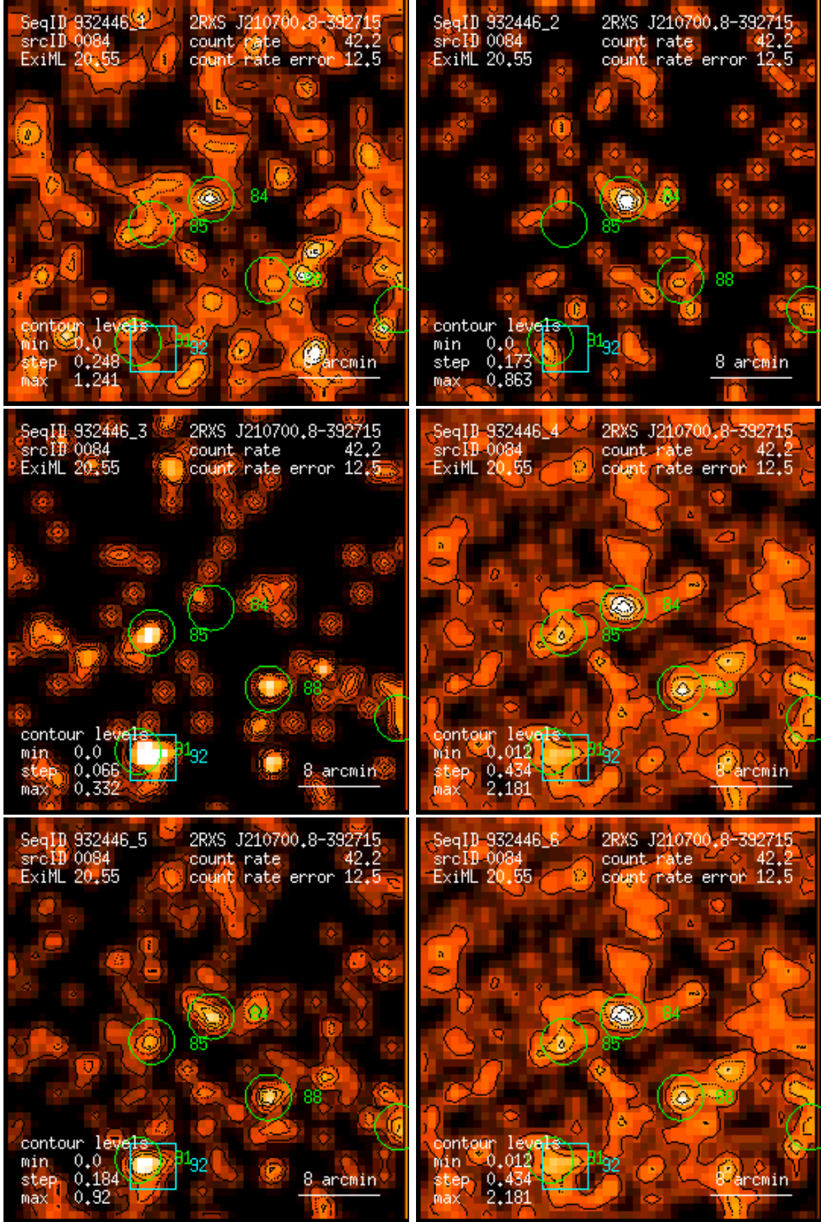
Figure 84: RASS 932446: detection 0084: band rate images, Gaussian filter: (1) PSPC channels 11 – 41, (2) 52 – 90, (3) 91 – 201, (4) 11 – 235, (5) 52 – 201, (6) 11 – 201. Broad band rates in counts/ks. Band rate contour levels in counts/ks/arcmin 2 .
