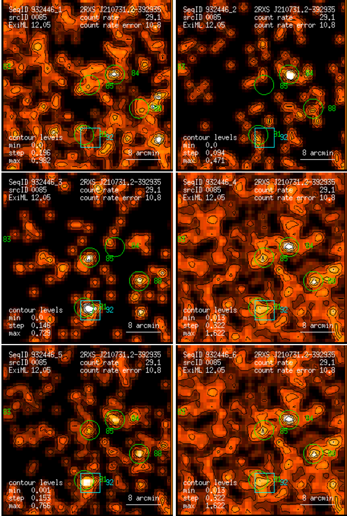
Figure 85: RASS 932446: detection 0085: band rate images, Gaussian filter: (1) PSPC channels 11 – 41, (2) 52 – 90, (3) 91 – 201, (4) 11 – 235, (5) 52 – 201, (6) 11 – 201. Broad band rates in counts/ks. Band rate contour levels in counts/ks/arcmin 2 .
