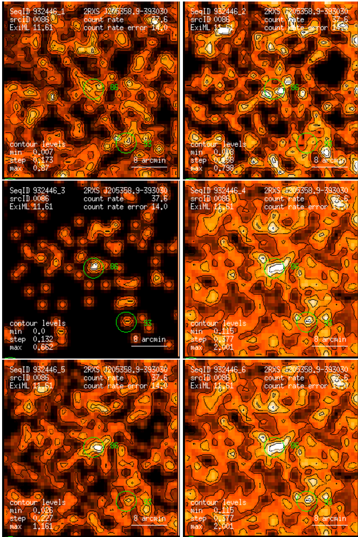
Figure 86: RASS 932446: detection 0086: band rate images, Gaussian filter: (1) PSPC channels 11 – 41, (2) 52 – 90, (3) 91 – 201, (4) 11 – 235, (5) 52 – 201, (6) 11 – 201. Broad band rates in counts/ks. Band rate contour levels in counts/ks/arcmin 2 .
