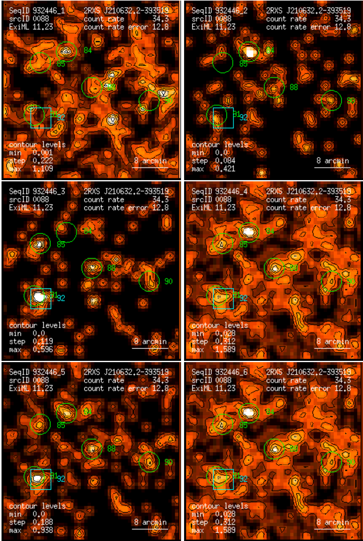
Figure 88: RASS 932446: detection 0088: band rate images, Gaussian filter: (1) PSPC channels 11 – 41, (2) 52 – 90, (3) 91 – 201, (4) 11 – 235, (5) 52 – 201, (6) 11 – 201. Broad band rates in counts/ks. Band rate contour levels in counts/ks/arcmin 2 .
