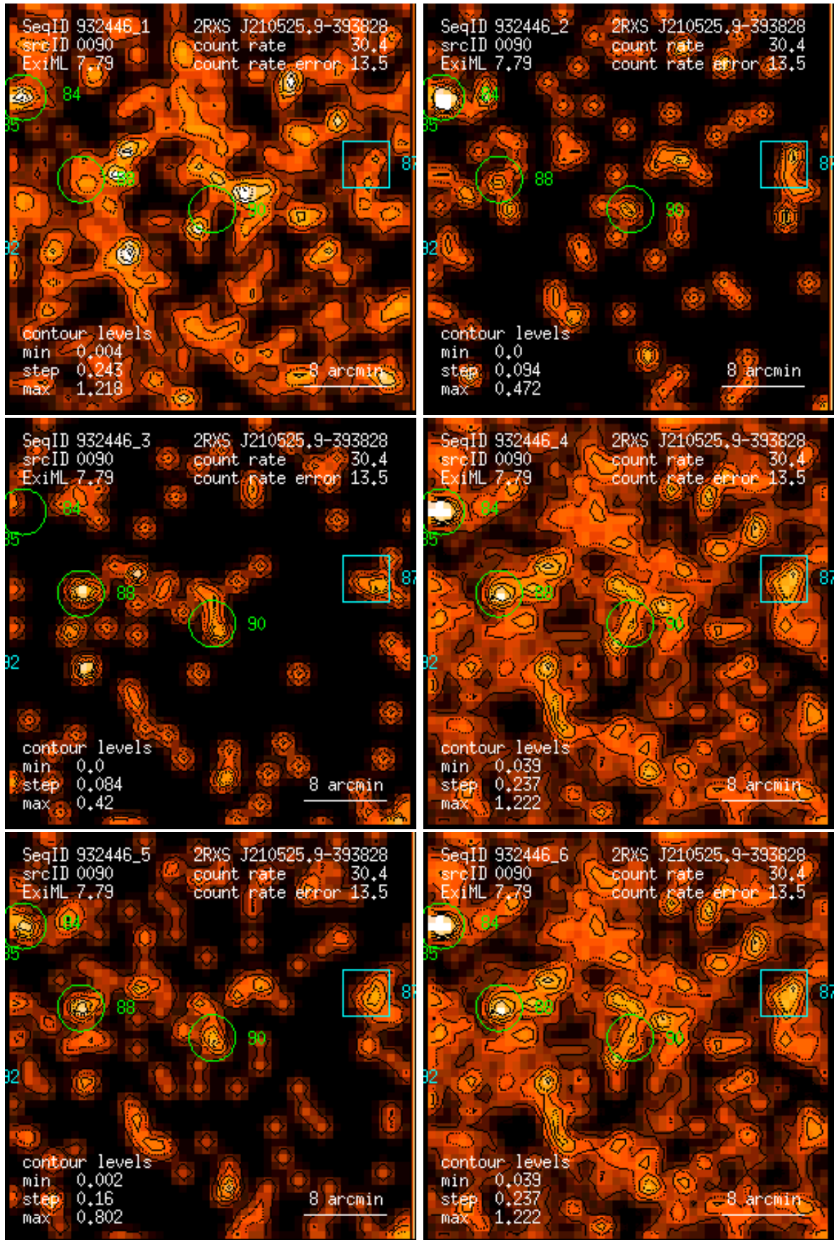
Figure 90: RASS 932446: detection 0090: band rate images, Gaussian filter: (1) PSPC channels 11 – 41, (2) 52 – 90, (3) 91 – 201, (4) 11 – 235, (5) 52 – 201, (6) 11 – 201. Broad band rates in counts/ks. Band rate contour levels in counts/ks/arcmin 2 .
