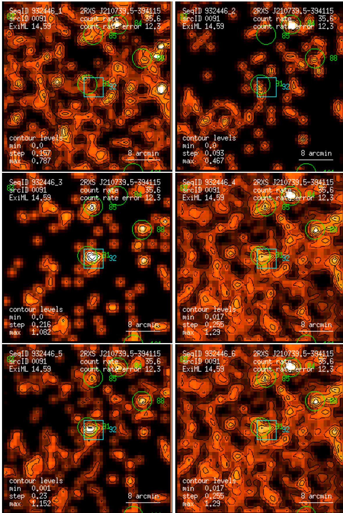
Figure 91: RASS 932446: detection 0091: band rate images, Gaussian filter: (1) PSPC channels 11 – 41, (2) 52 – 90, (3) 91 – 201, (4) 11 – 235, (5) 52 – 201, (6) 11 – 201. Broad band rates in counts/ks. Band rate contour levels in counts/ks/arcmin 2 .
