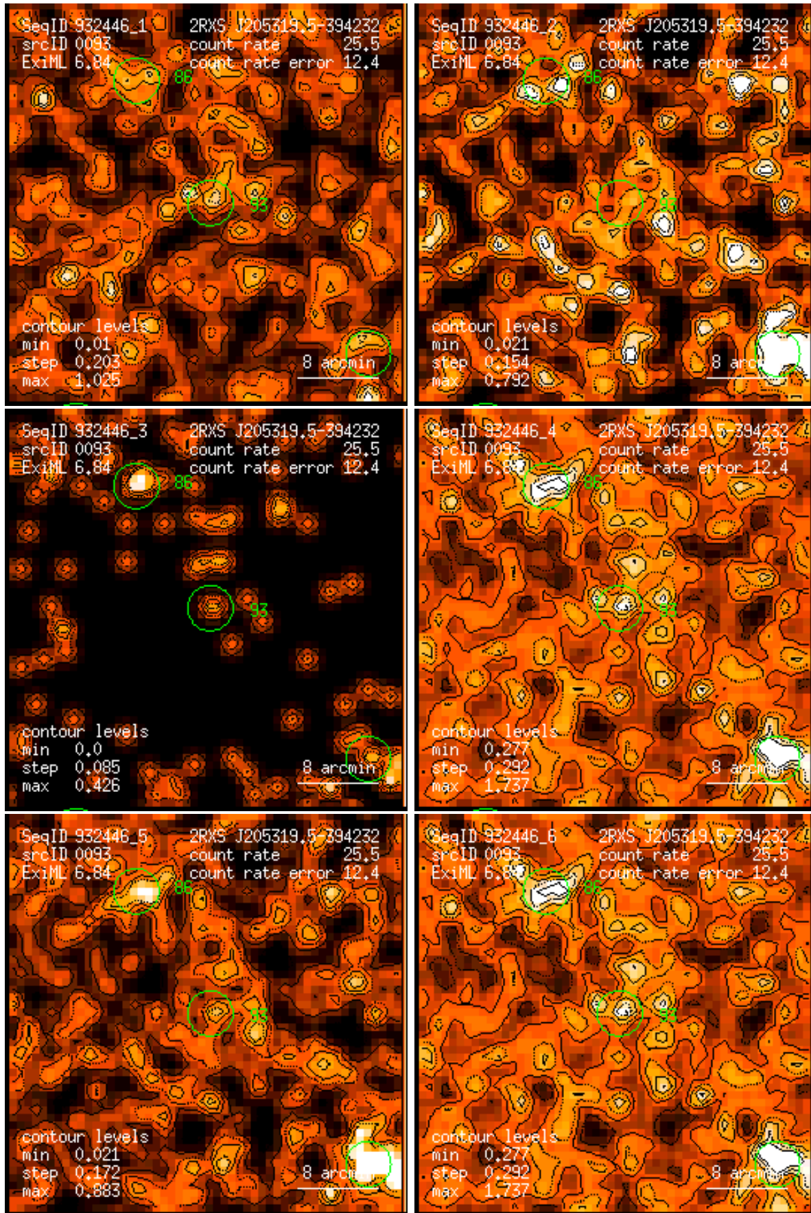
Figure 93: RASS 932446: detection 0093: band rate images, Gaussian filter: (1) PSPC channels 11 – 41, (2) 52 – 90, (3) 91 – 201, (4) 11 – 235, (5) 52 – 201, (6) 11 – 201. Broad band rates in counts/ks. Band rate contour levels in counts/ks/arcmin 2 .
