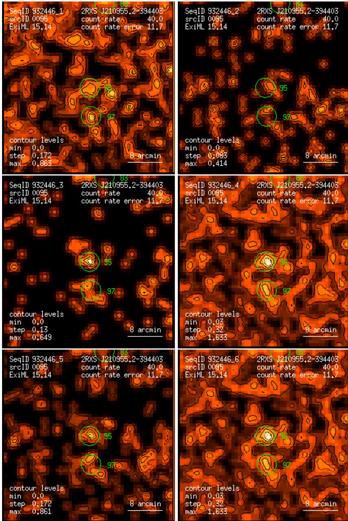
Figure 95: RASS 932446: detection 0095: band rate images, Gaussian filter: (1) PSPC channels 11 – 41, (2) 52 – 90, (3) 91 – 201, (4) 11 – 235, (5) 52 – 201, (6) 11 – 201. Broad band rates in counts/ks. Band rate contour levels in counts/ks/arcmin 2 .
