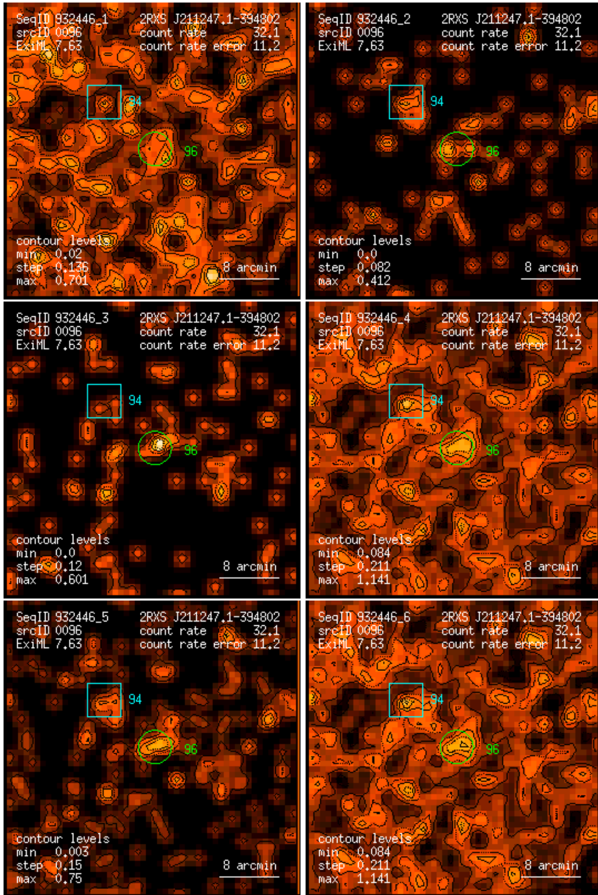
Figure 96: RASS 932446: detection 0096: band rate images, Gaussian filter: (1) PSPC channels 11 – 41, (2) 52 – 90, (3) 91 – 201, (4) 11 – 235, (5) 52 – 201, (6) 11 – 201. Broad band rates in counts/ks. Band rate contour levels in counts/ks/arcmin 2 .
