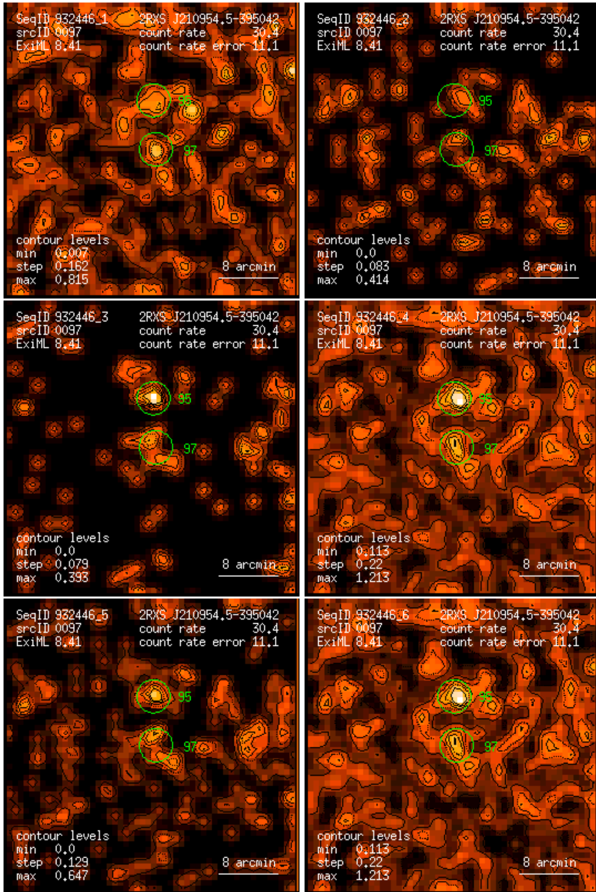
Figure 97: RASS 932446: detection 0097: band rate images, Gaussian filter: (1) PSPC channels 11 – 41, (2) 52 – 90, (3) 91 – 201, (4) 11 – 235, (5) 52 – 201, (6) 11 – 201. Broad band rates in counts/ks. Band rate contour levels in counts/ks/arcmin 2 .
