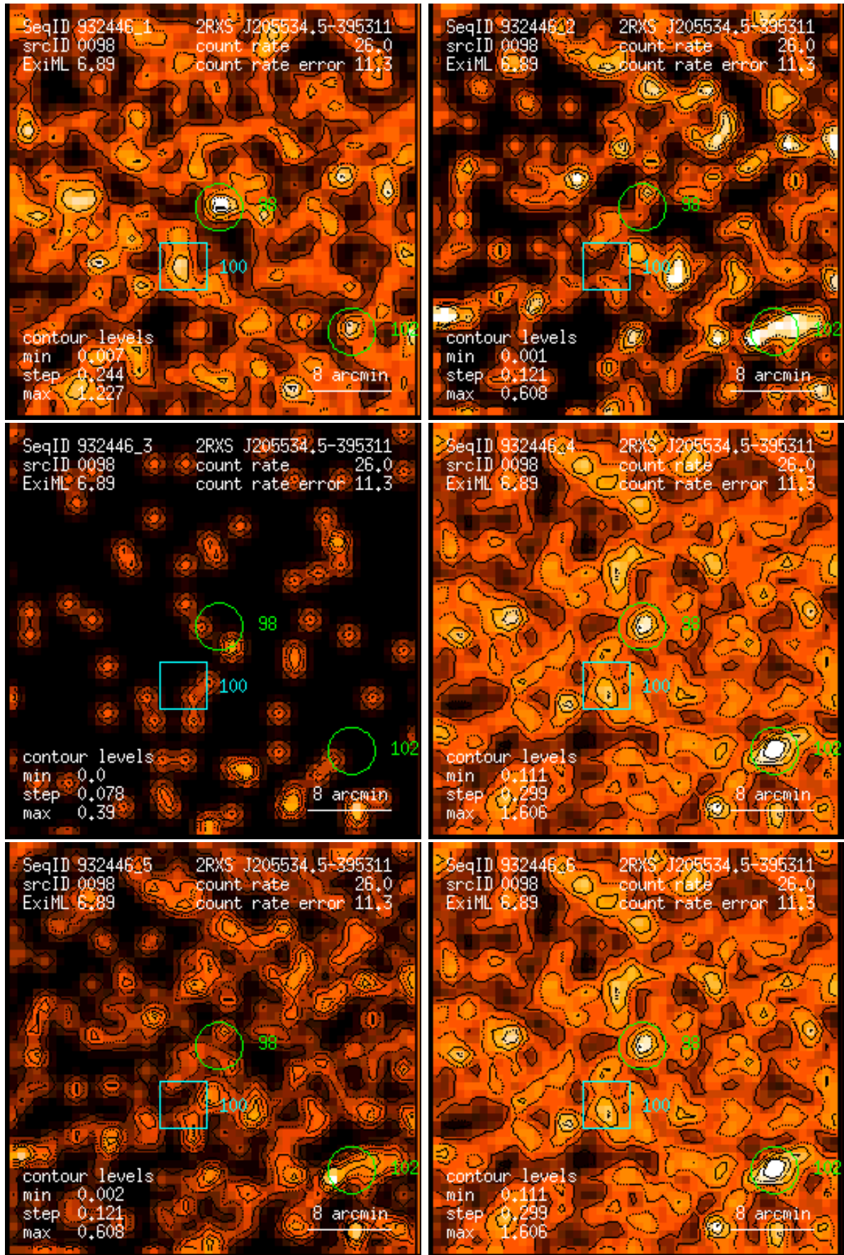
Figure 98: RASS 932446: detection 0098: band rate images, Gaussian filter: (1) PSPC channels 11 – 41, (2) 52 – 90, (3) 91 – 201, (4) 11 – 235, (5) 52 – 201, (6) 11 – 201. Broad band rates in counts/ks. Band rate contour levels in counts/ks/arcmin 2 .
