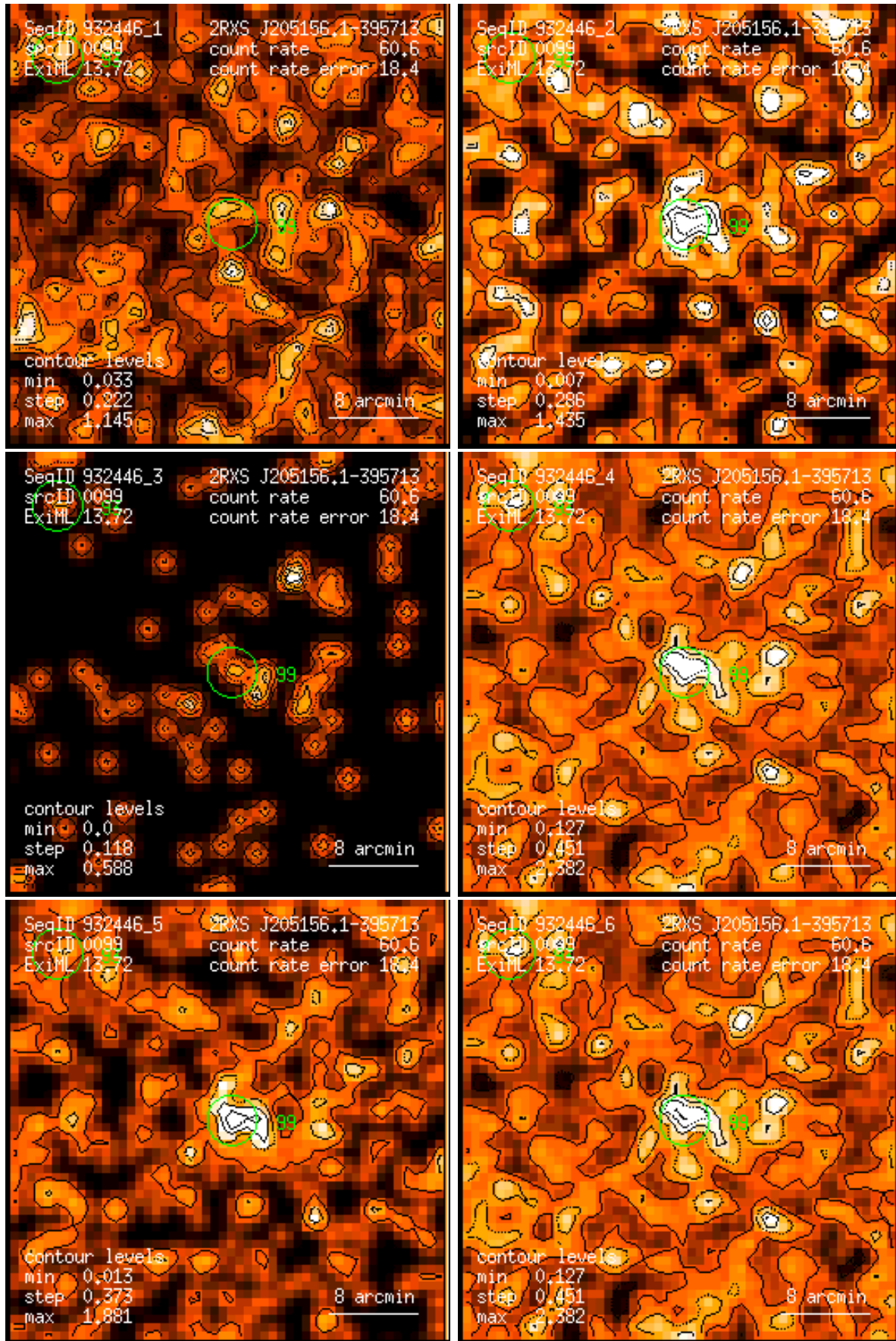
Figure 99: RASS 932446: detection 0099: band rate images, Gaussian filter: (1) PSPC channels 11 – 41, (2) 52 – 90, (3) 91 – 201, (4) 11 – 235, (5) 52 – 201, (6) 11 – 201. Broad band rates in counts/ks. Band rate contour levels in counts/ks/arcmin 2 .
