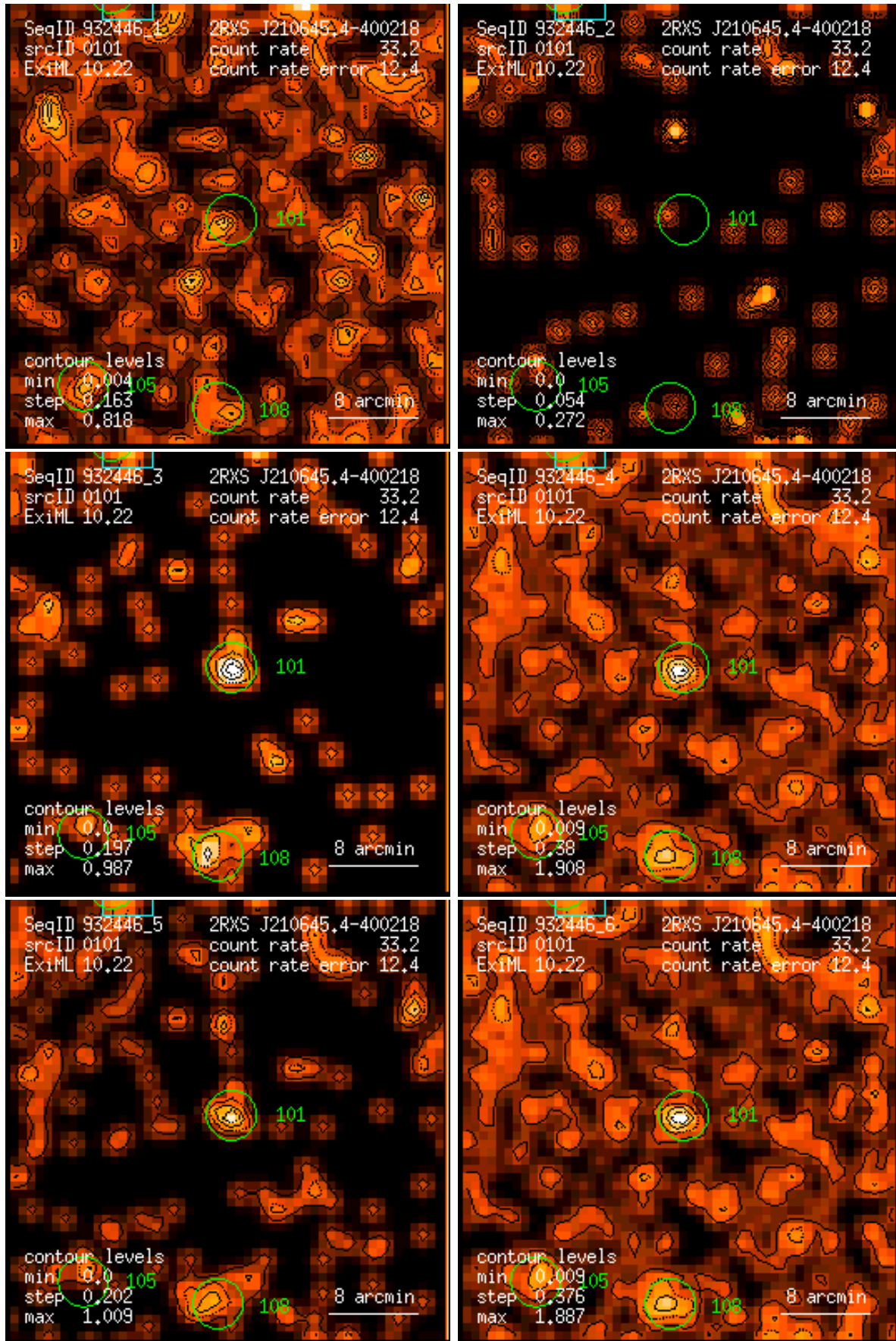
Figure 101: RASS 932446: detection 0101: band rate images, Gaussian filter: (1) PSPC channels 11 – 41, (2) 52 – 90, (3) 91 – 201, (4) 11 – 235, (5) 52 – 201, (6) 11 – 201. Broad band rates in counts/ks. Band rate contour levels in counts/ks/arcmin 2 .
