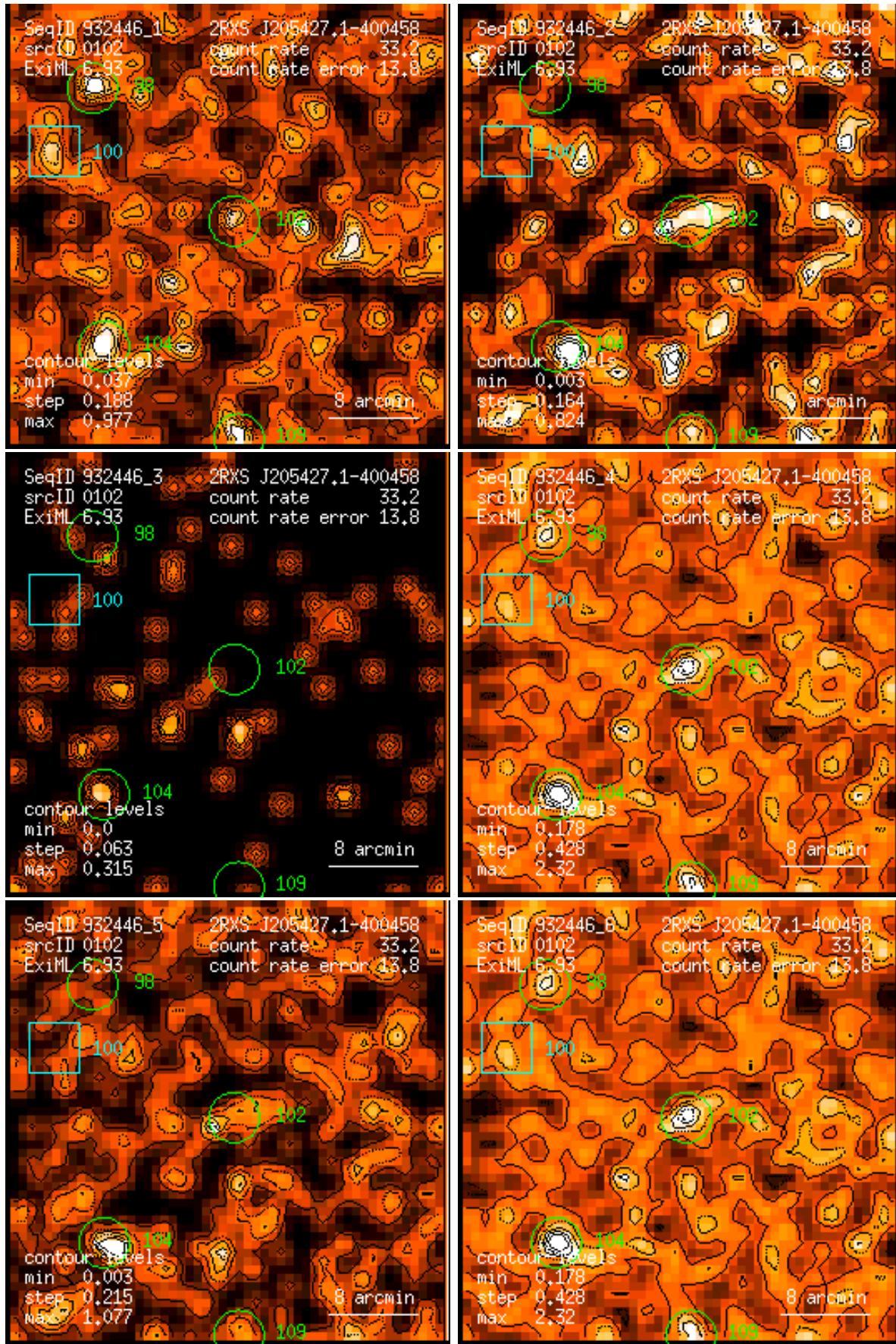
Figure 102: RASS 932446: detection 0102: band rate images, Gaussian filter: (1) PSPC channels 11 – 41, (2) 52 – 90, (3) 91 – 201, (4) 11 – 235, (5) 52 – 201, (6) 11 – 201. Broad band rates in counts/ks. Band rate contour levels in counts/ks/arcmin 2 .
