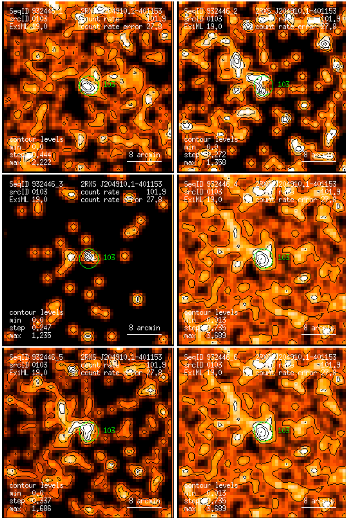
Figure 103: RASS 932446: detection 0103: band rate images, Gaussian filter: (1) PSPC channels 11 – 41, (2) 52 – 90, (3) 91 – 201, (4) 11 – 235, (5) 52 – 201, (6) 11 – 201. Broad band rates in counts/ks. Band rate contour levels in counts/ks/arcmin 2 .
