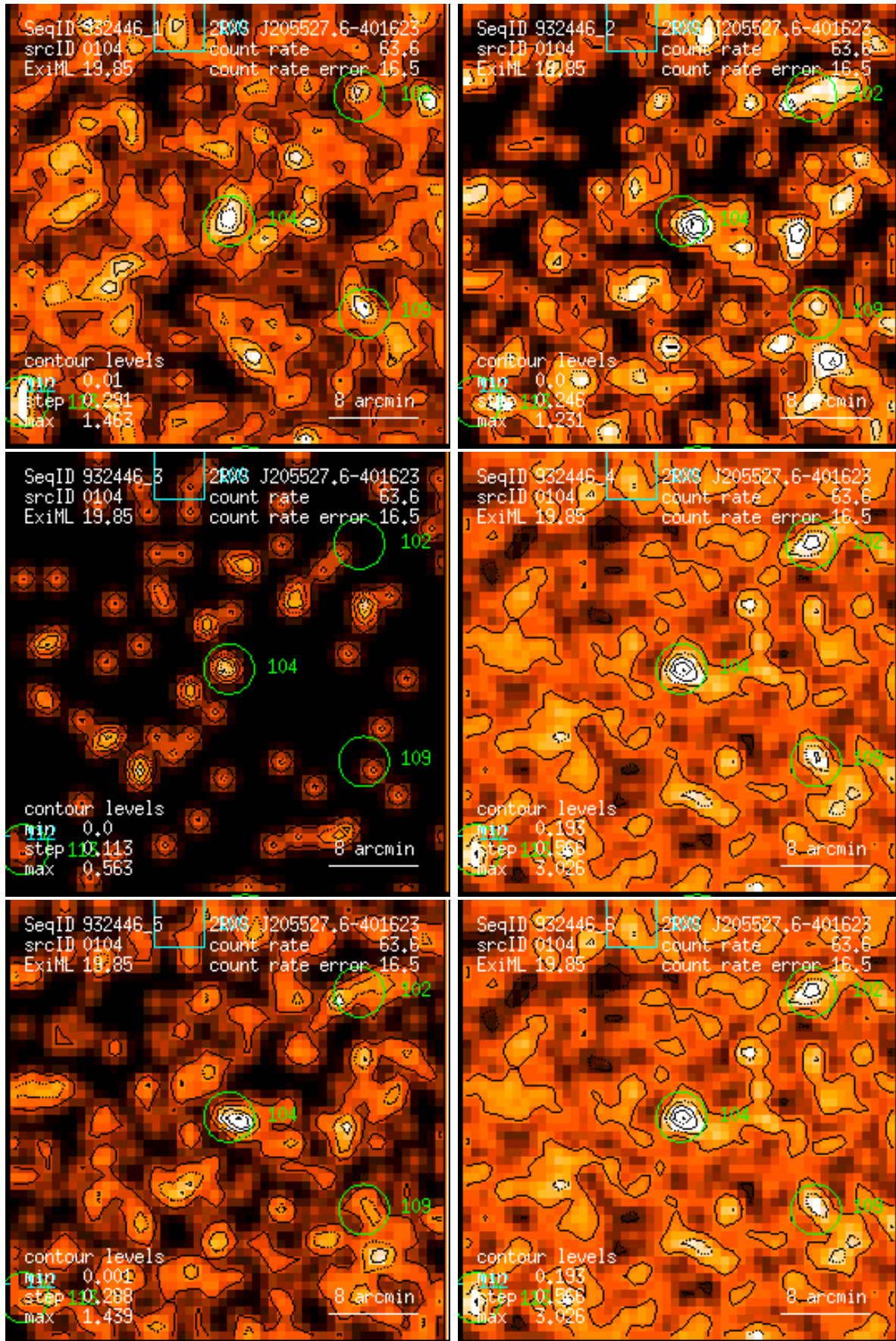
Figure 104: RASS 932446: detection 0104: band rate images, Gaussian filter: (1) PSPC channels 11 – 41, (2) 52 – 90, (3) 91 – 201, (4) 11 – 235, (5) 52 – 201, (6) 11 – 201. Broad band rates in counts/ks. Band rate contour levels in counts/ks/arcmin 2 .
