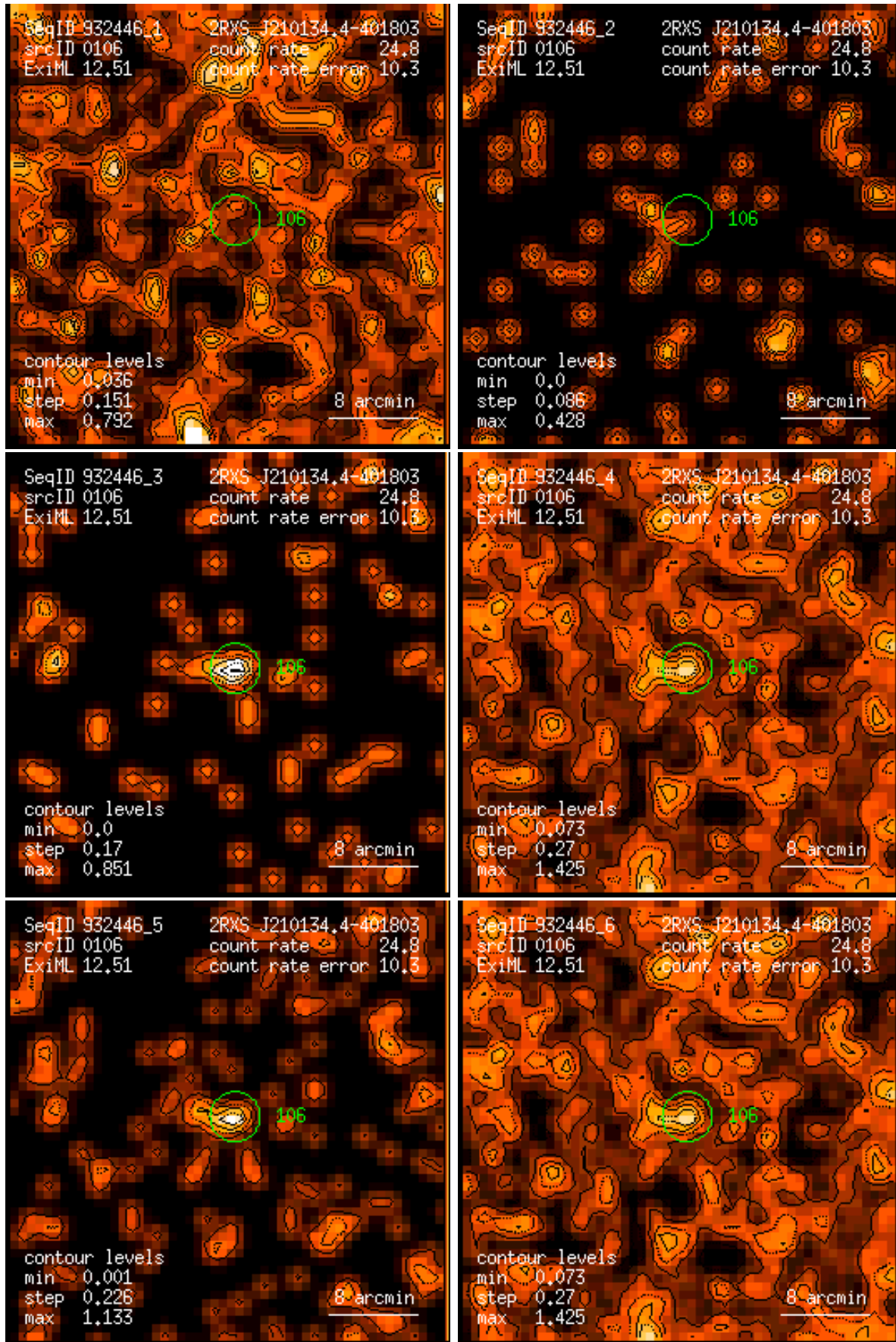
Figure 106: RASS 932446: detection 0106: band rate images, Gaussian filter: (1) PSPC channels 11 – 41, (2) 52 – 90, (3) 91 – 201, (4) 11 – 235, (5) 52 – 201, (6) 11 – 201. Broad band rates in counts/ks. Band rate contour levels in counts/ks/arcmin 2 .
