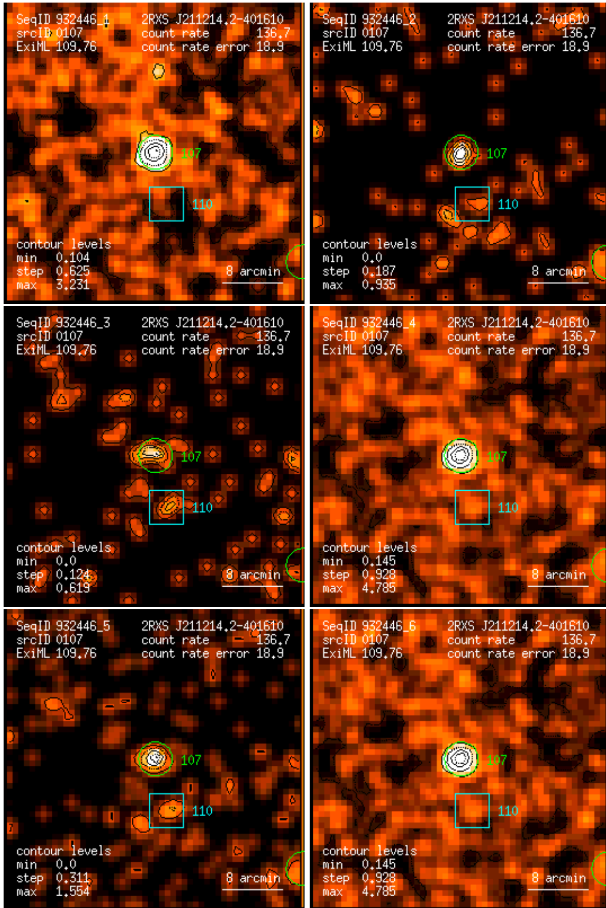
Figure 107: RASS 932446: detection 0107: band rate images, Gaussian filter: (1) PSPC channels 11 – 41, (2) 52 – 90, (3) 91 – 201, (4) 11 – 235, (5) 52 – 201, (6) 11 – 201. Broad band rates in counts/ks. Band rate contour levels in counts/ks/arcmin 2 .
