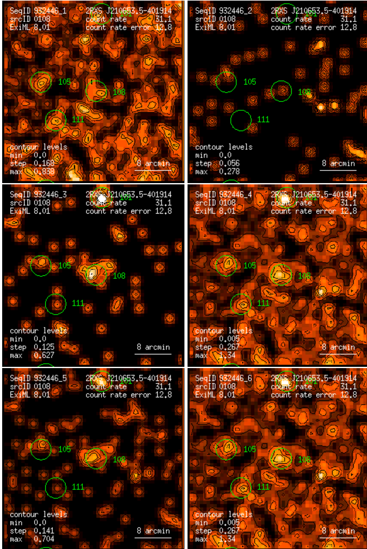
Figure 108: RASS 932446: detection 0108: band rate images, Gaussian filter: (1) PSPC channels 11 – 41, (2) 52 – 90, (3) 91 – 201, (4) 11 – 235, (5) 52 – 201, (6) 11 – 201. Broad band rates in counts/ks. Band rate contour levels in counts/ks/arcmin 2 .
