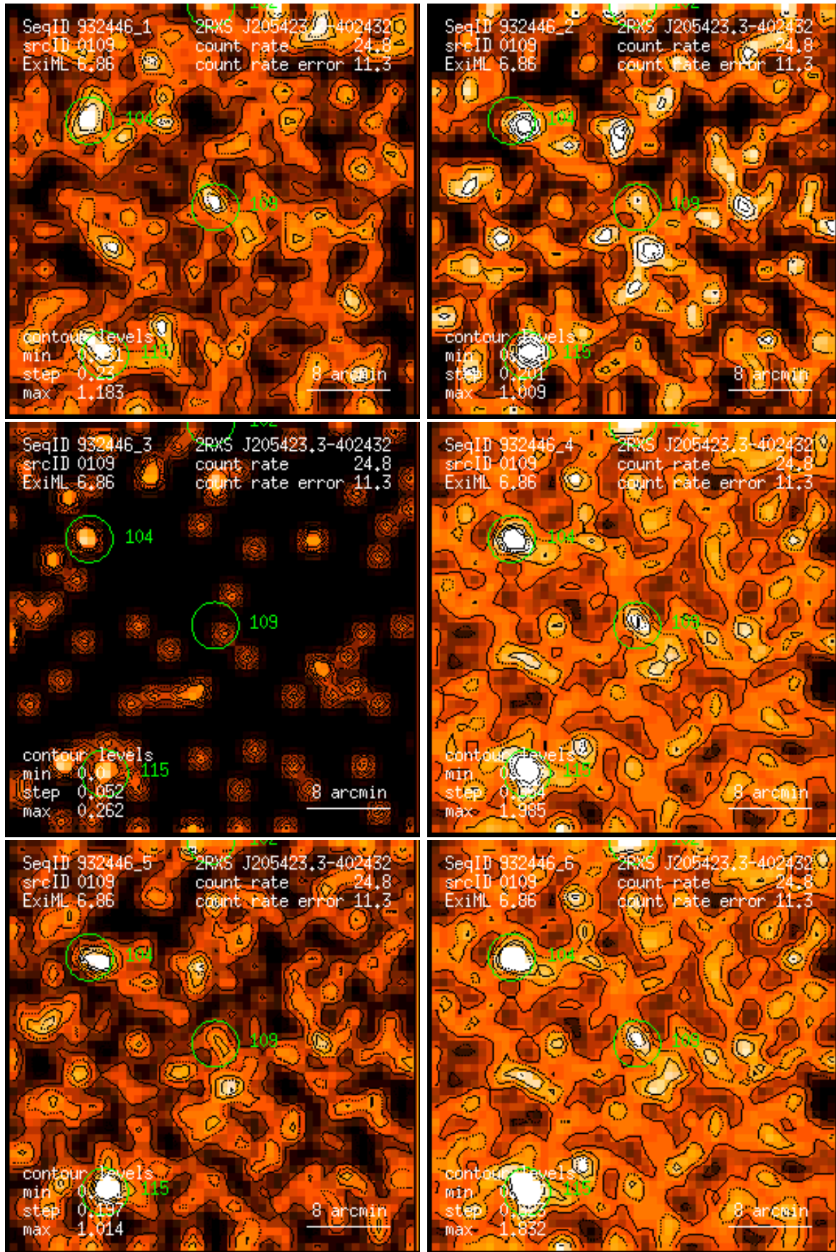
Figure 109: RASS 932446: detection 0109: band rate images, Gaussian filter: (1) PSPC channels 11 – 41, (2) 52 – 90, (3) 91 – 201, (4) 11 – 235, (5) 52 – 201, (6) 11 – 201. Broad band rates in counts/ks. Band rate contour levels in counts/ks/arcmin 2 .
