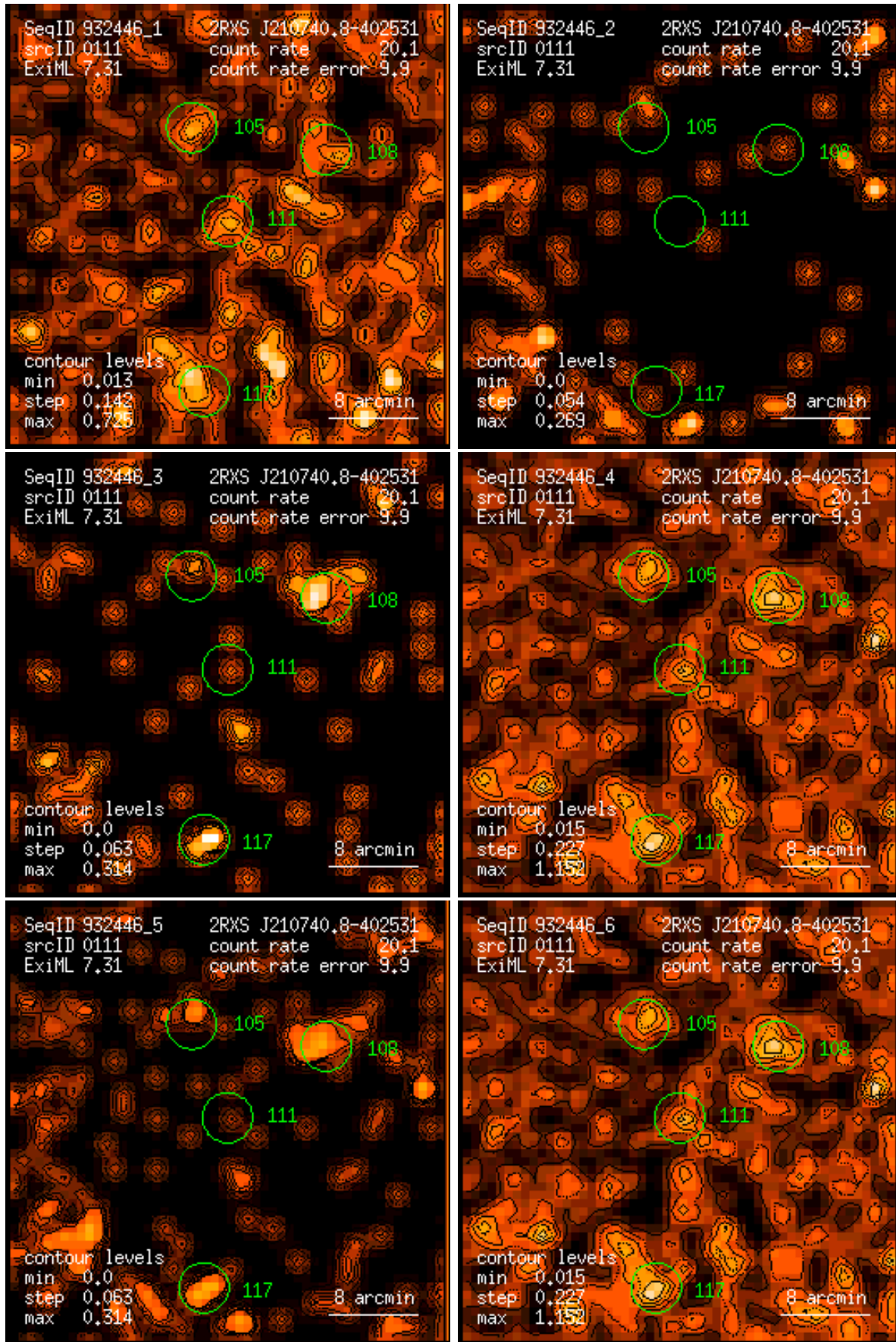
Figure 111: RASS 932446: detection 0111: band rate images, Gaussian filter: (1) PSPC channels 11 – 41, (2) 52 – 90, (3) 91 – 201, (4) 11 – 235, (5) 52 – 201, (6) 11 – 201. Broad band rates in counts/ks. Band rate contour levels in counts/ks/arcmin 2 .
