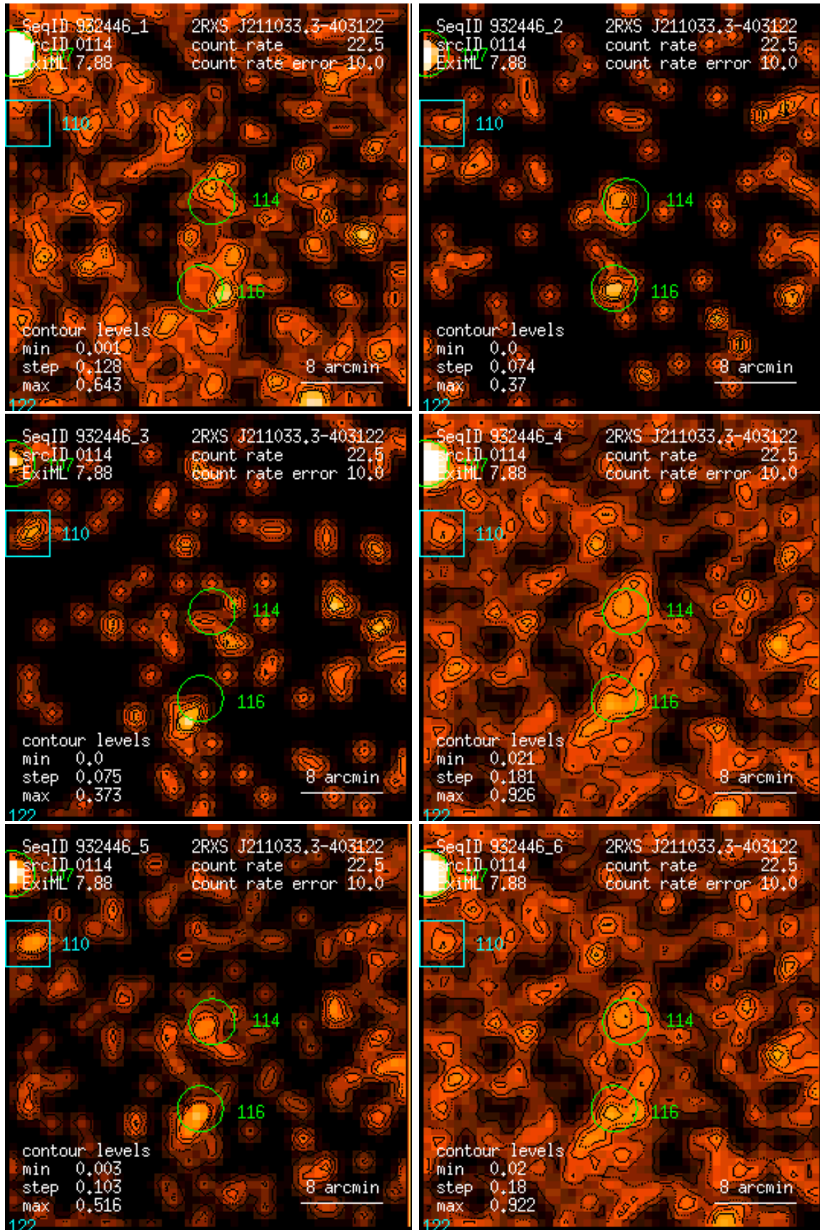
Figure 114: RASS 932446: detection 0114: band rate images, Gaussian filter: (1) PSPC channels 11 – 41, (2) 52 – 90, (3) 91 – 201, (4) 11 – 235, (5) 52 – 201, (6) 11 – 201. Broad band rates in counts/ks. Band rate contour levels in counts/ks/arcmin 2 .
