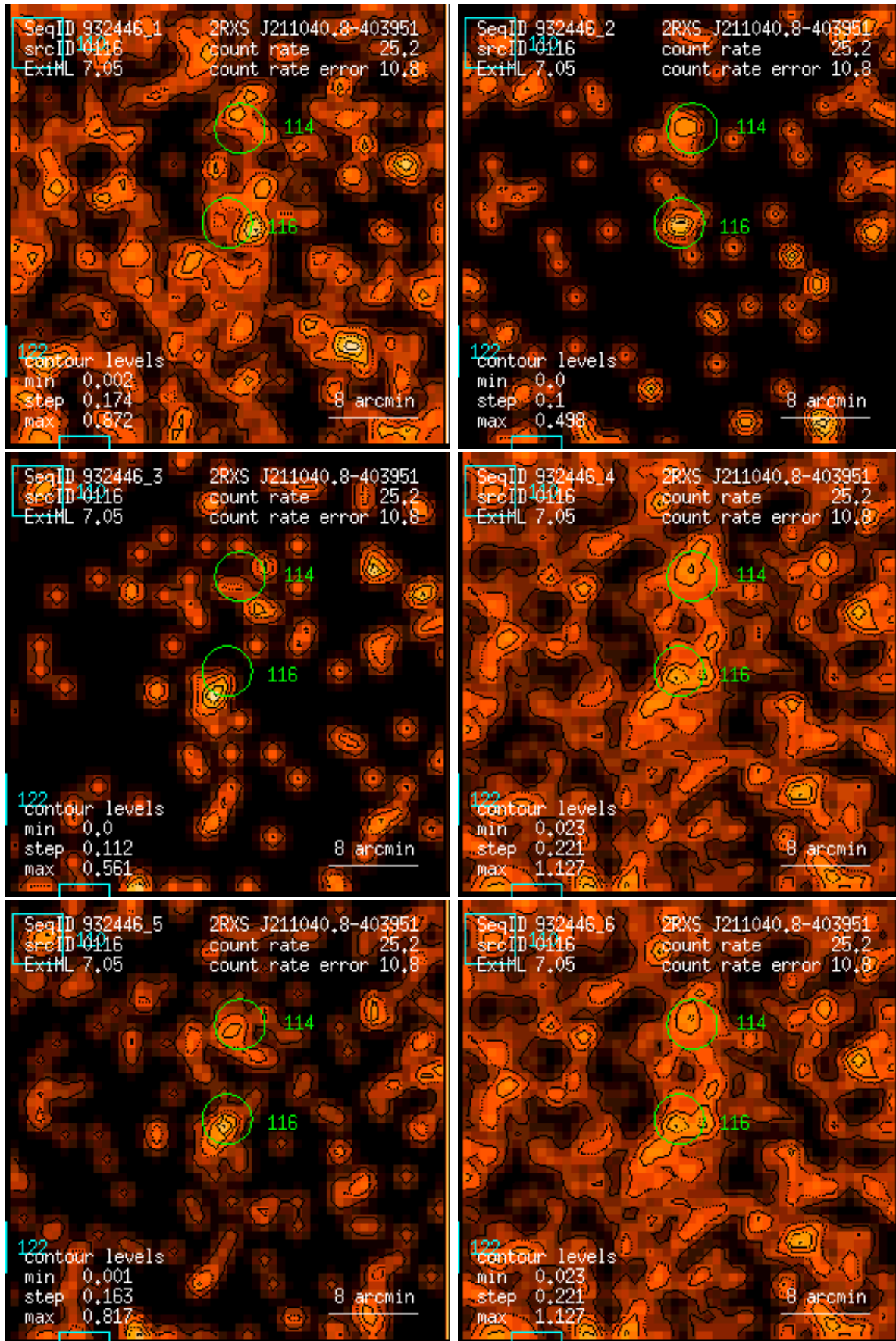
Figure 116: RASS 932446: detection 0116: band rate images, Gaussian filter: (1) PSPC channels 11 – 41, (2) 52 – 90, (3) 91 – 201, (4) 11 – 235, (5) 52 – 201, (6) 11 – 201. Broad band rates in counts/ks. Band rate contour levels in counts/ks/arcmin 2 .
