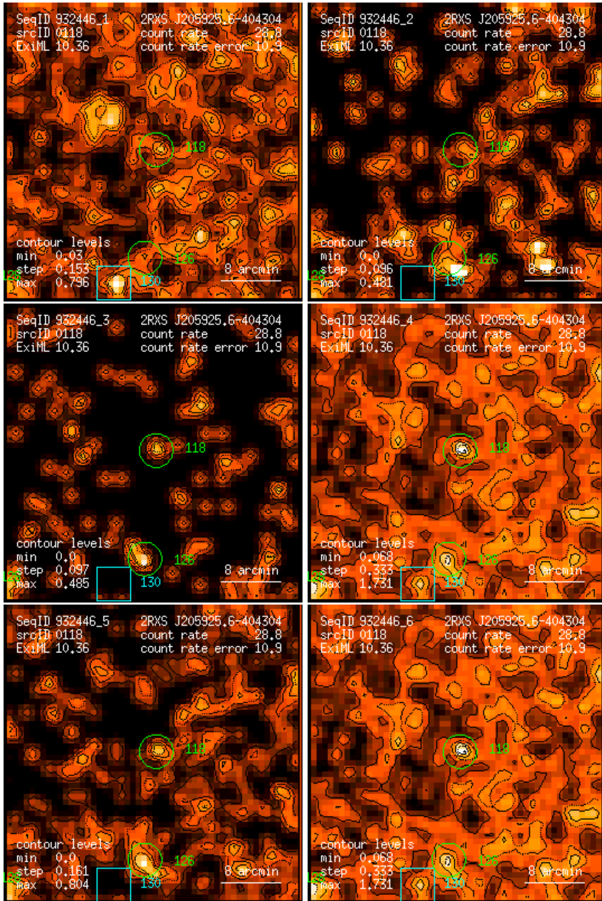
Figure 118: RASS 932446: detection 0118: band rate images, Gaussian filter: (1) PSPC channels 11 – 41, (2) 52 – 90, (3) 91 – 201, (4) 11 – 235, (5) 52 – 201, (6) 11 – 201. Broad band rates in counts/ks. Band rate contour levels in counts/ks/arcmin 2 .
