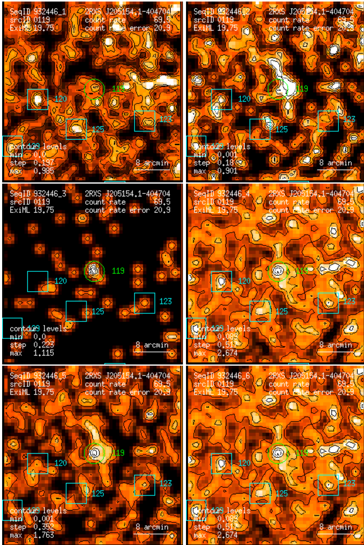
Figure 119: RASS 932446: detection 0119: band rate images, Gaussian filter: (1) PSPC channels 11 – 41, (2) 52 – 90, (3) 91 – 201, (4) 11 – 235, (5) 52 – 201, (6) 11 – 201. Broad band rates in counts/ks. Band rate contour levels in counts/ks/arcmin 2 .
