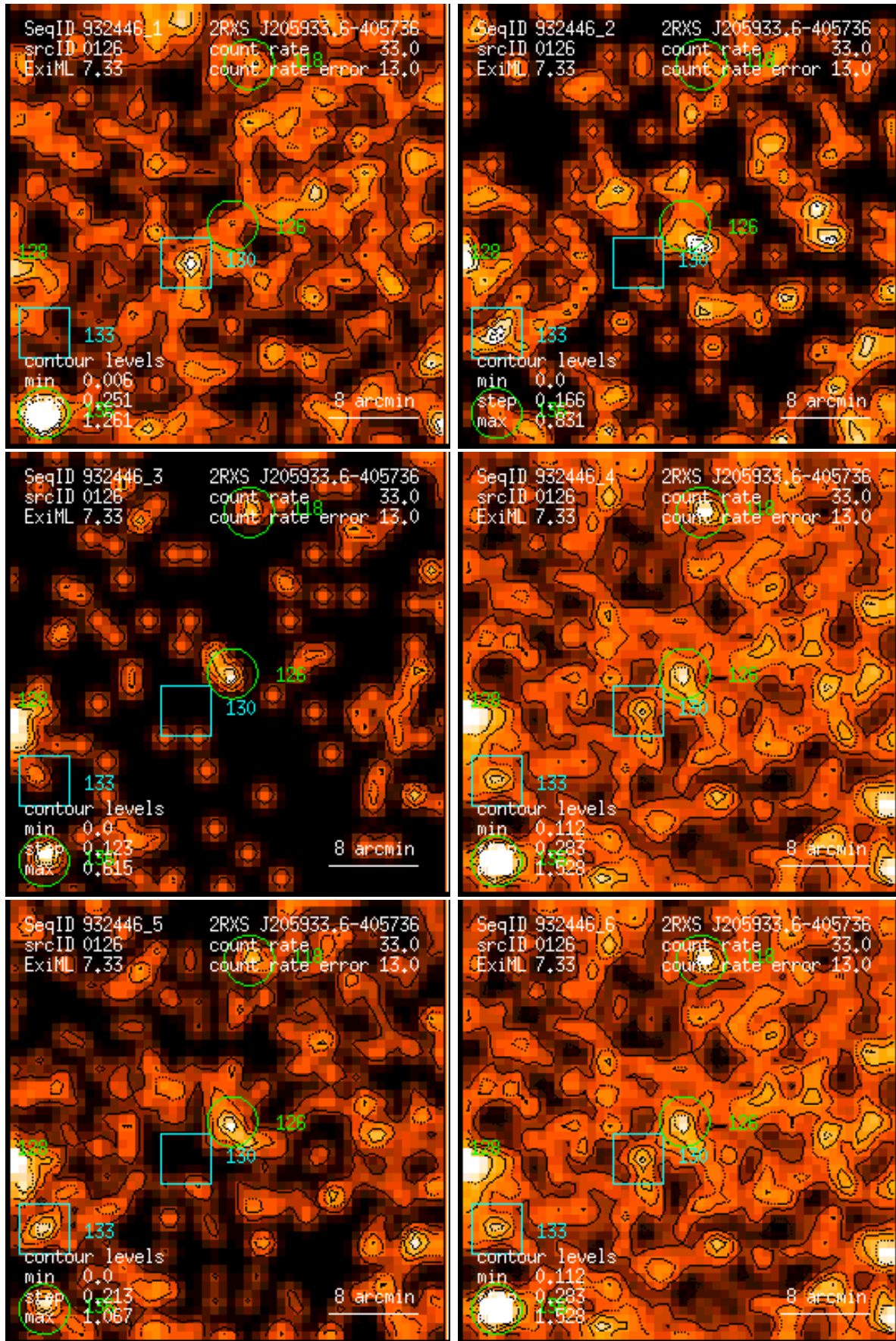
Figure 126: RASS 932446: detection 0126: band rate images, Gaussian filter: (1) PSPC channels 11 – 41, (2) 52 – 90, (3) 91 – 201, (4) 11 – 235, (5) 52 – 201, (6) 11 – 201. Broad band rates in counts/ks. Band rate contour levels in counts/ks/arcmin 2 .
