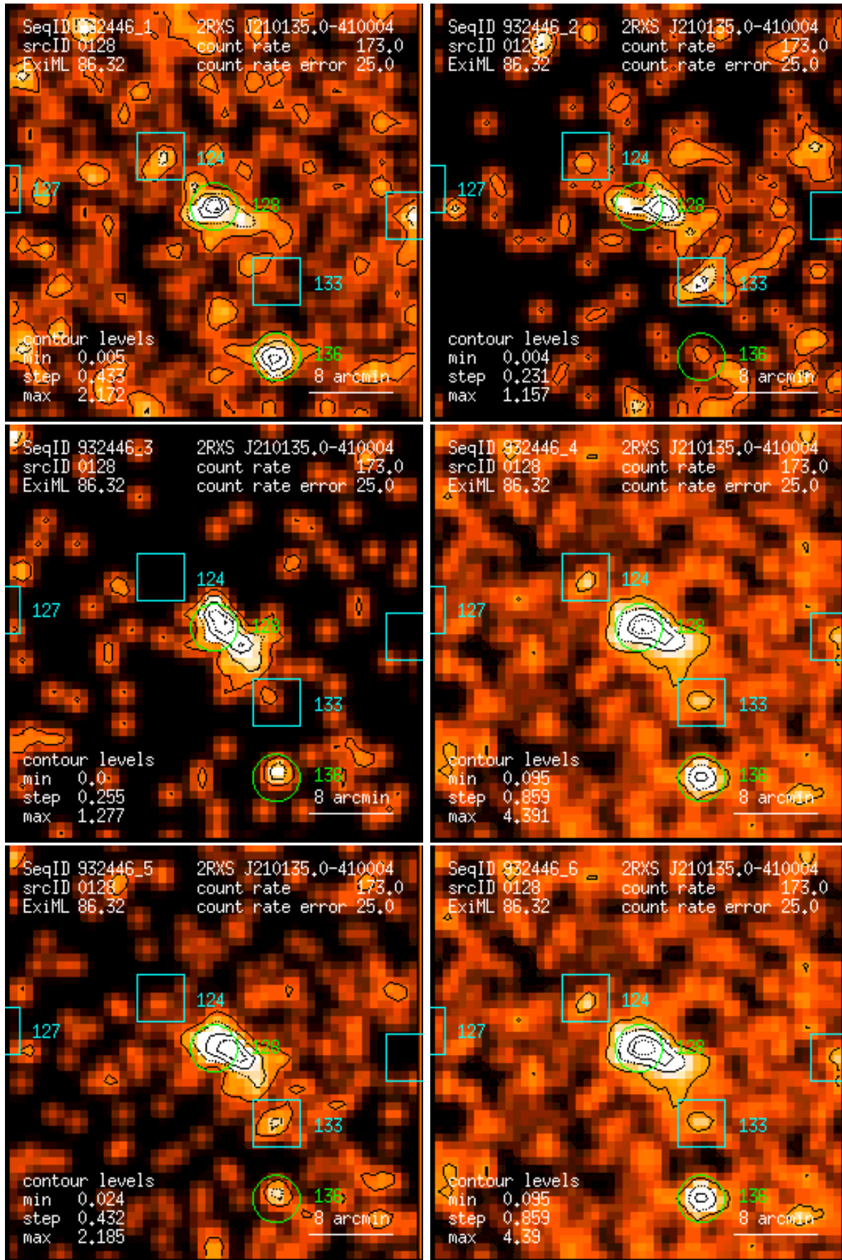
Figure 128: RASS 932446: detection 0128: band rate images, Gaussian filter: (1) PSPC channels 11 – 41, (2) 52 – 90, (3) 91 – 201, (4) 11 – 235, (5) 52 – 201, (6) 11 – 201. Broad band rates in counts/ks. Band rate contour levels in counts/ks/arcmin 2 .
