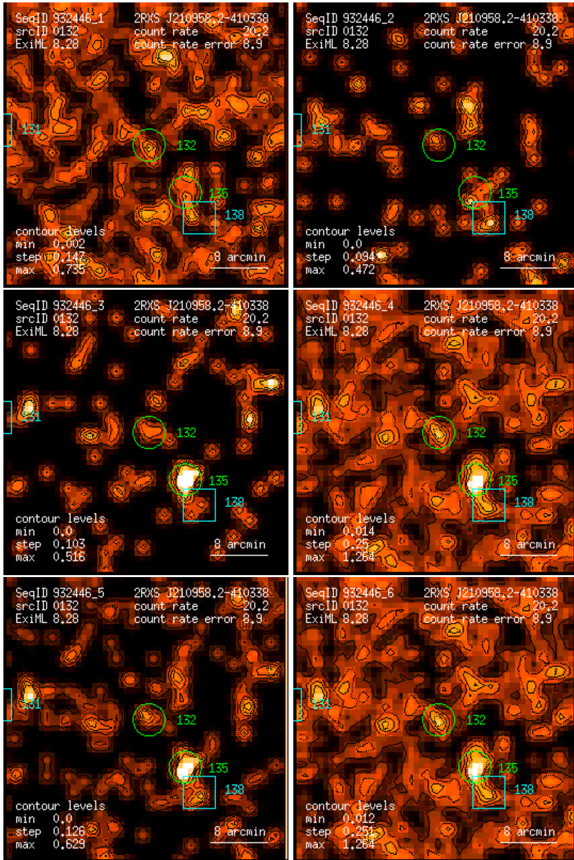
Figure 132: RASS 932446: detection 0132: band rate images, Gaussian filter: (1) PSPC channels 11 – 41, (2) 52 – 90, (3) 91 – 201, (4) 11 – 235, (5) 52 – 201, (6) 11 – 201. Broad band rates in counts/ks. Band rate contour levels in counts/ks/arcmin 2 .
