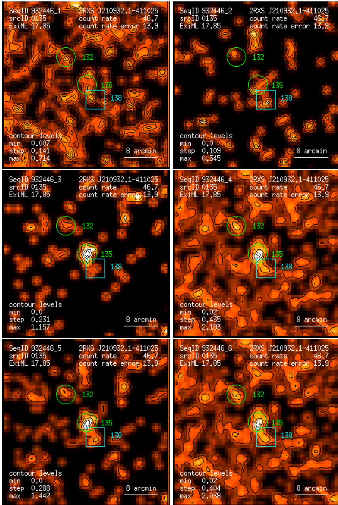
Figure 135: RASS 932446: detection 0135: band rate images, Gaussian filter: (1) PSPC channels 11 – 41, (2) 52 – 90, (3) 91 – 201, (4) 11 – 235, (5) 52 – 201, (6) 11 – 201. Broad band rates in counts/ks. Band rate contour levels in counts/ks/arcmin 2 .
