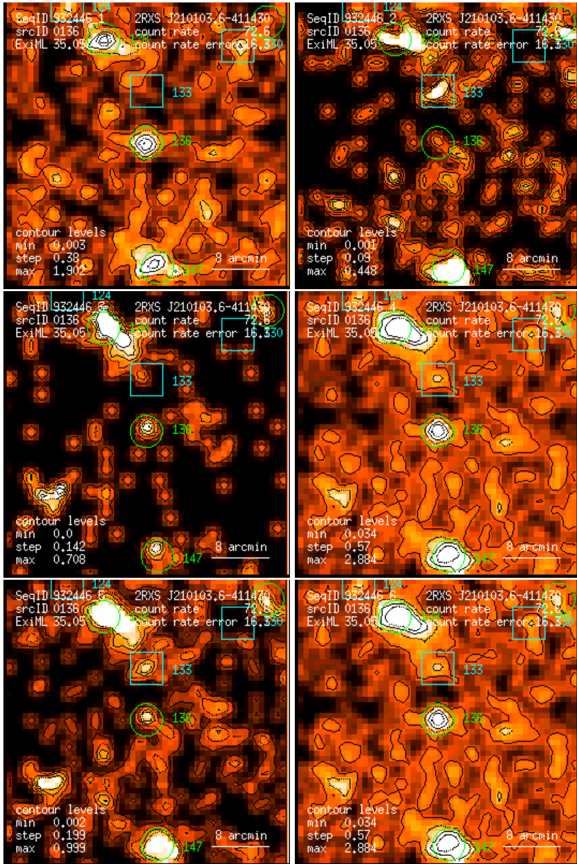
Figure 136: RASS 932446: detection 0136: band rate images, Gaussian filter: (1) PSPC channels 11 – 41, (2) 52 – 90, (3) 91 – 201, (4) 11 – 235, (5) 52 – 201, (6) 11 – 201. Broad band rates in counts/ks. Band rate contour levels in counts/ks/arcmin 2 .
